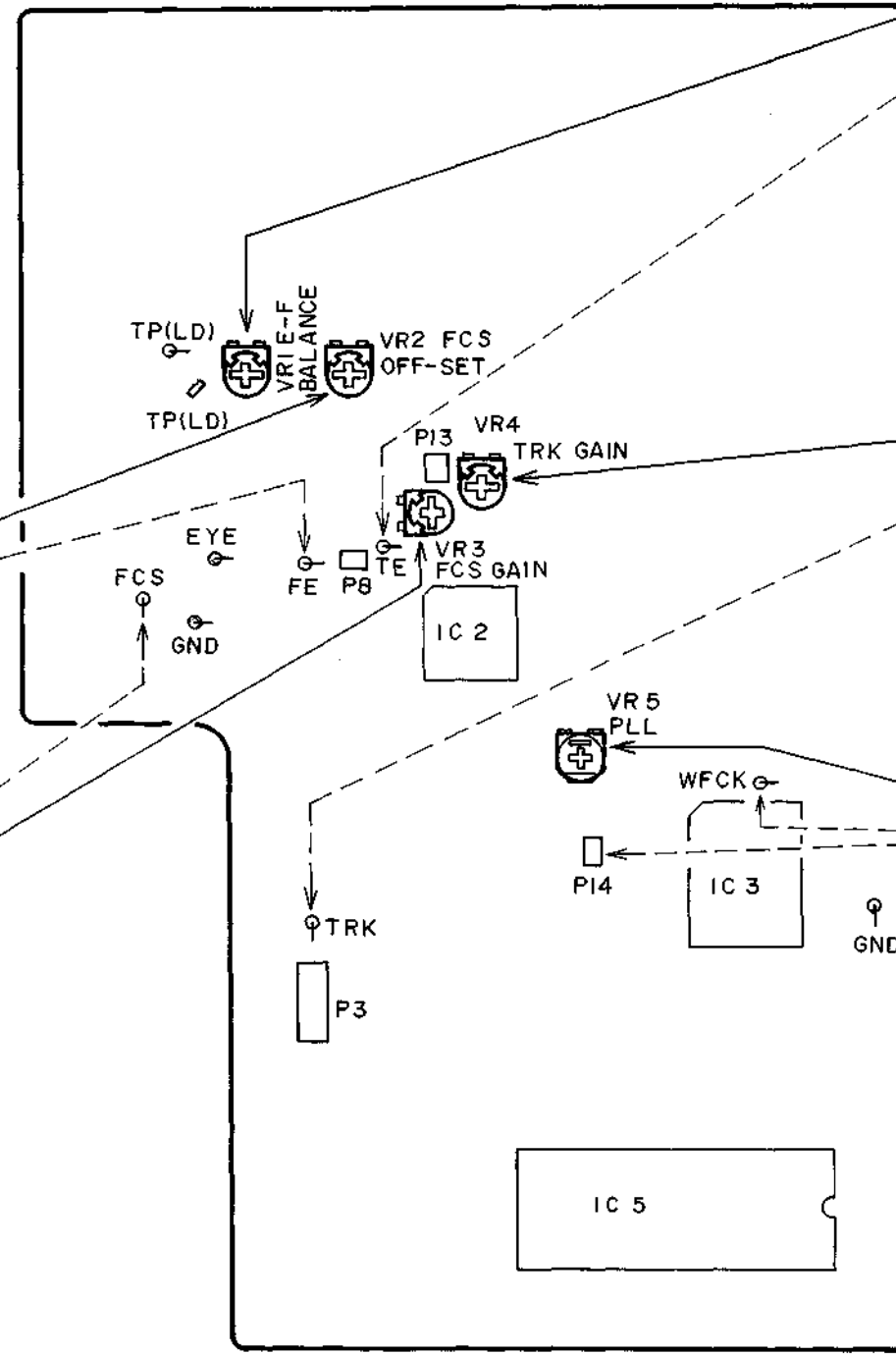
MAIN PCB
