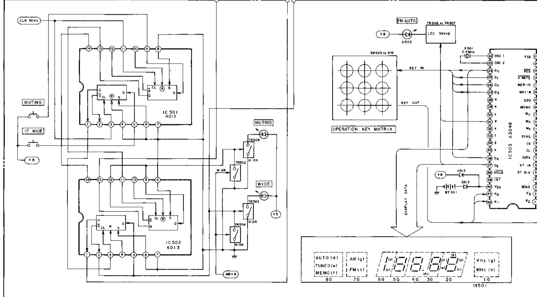
CONTROL BLOCK
