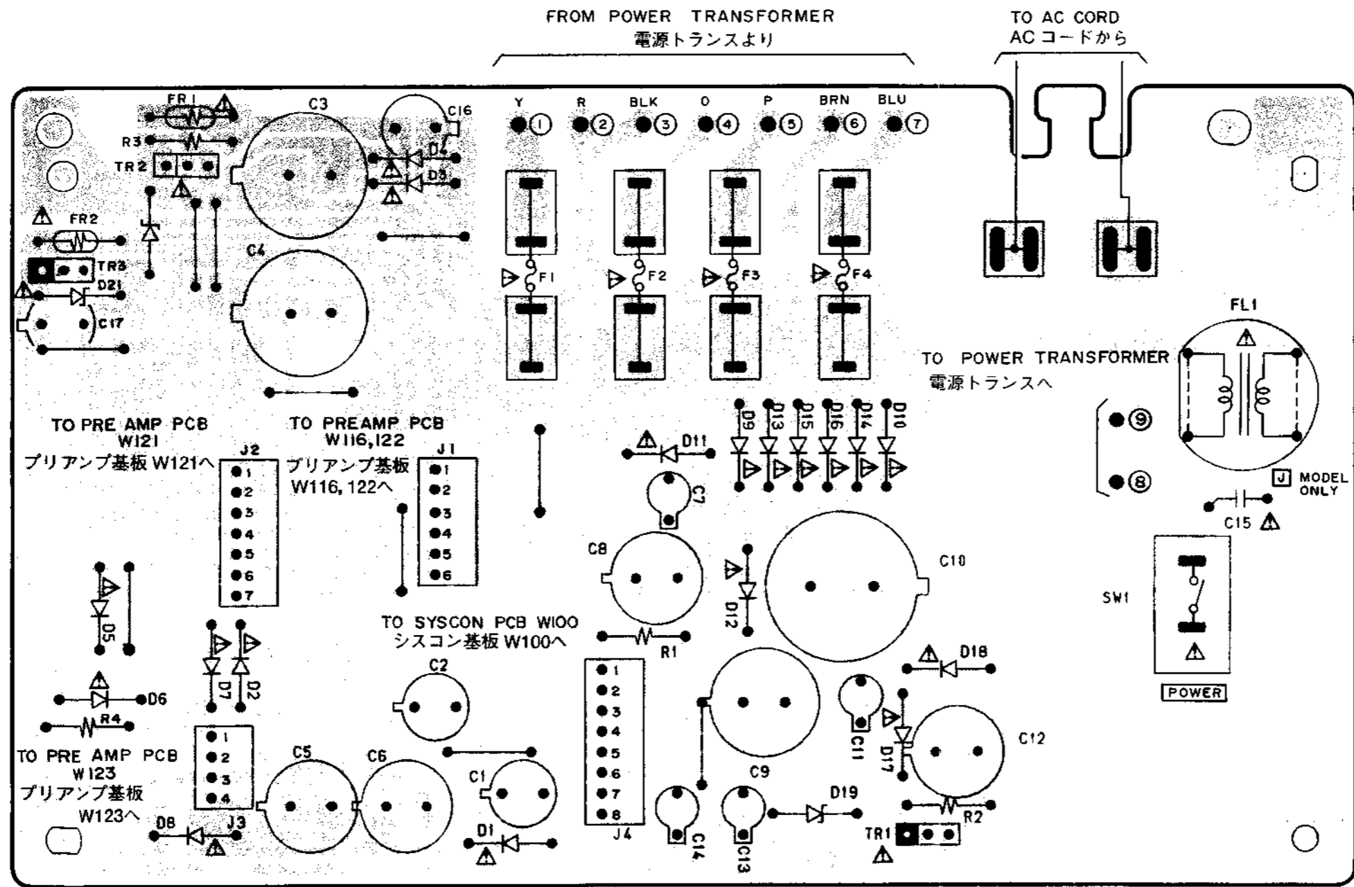
POWER SUPPLY PCB T2107C5030 電源基板
