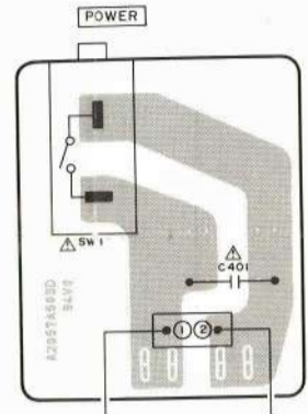
POWER SW PCB A2057A503D
