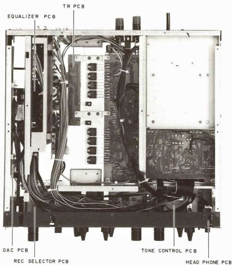
Fig. 3-2 Bottom View
