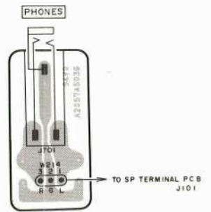
HEAD PHONE PCB A2057A503G
