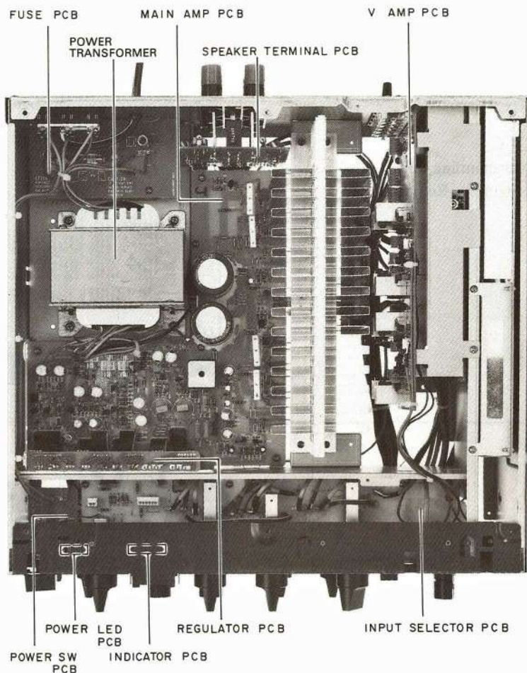
Fig. 3-1 Top View
