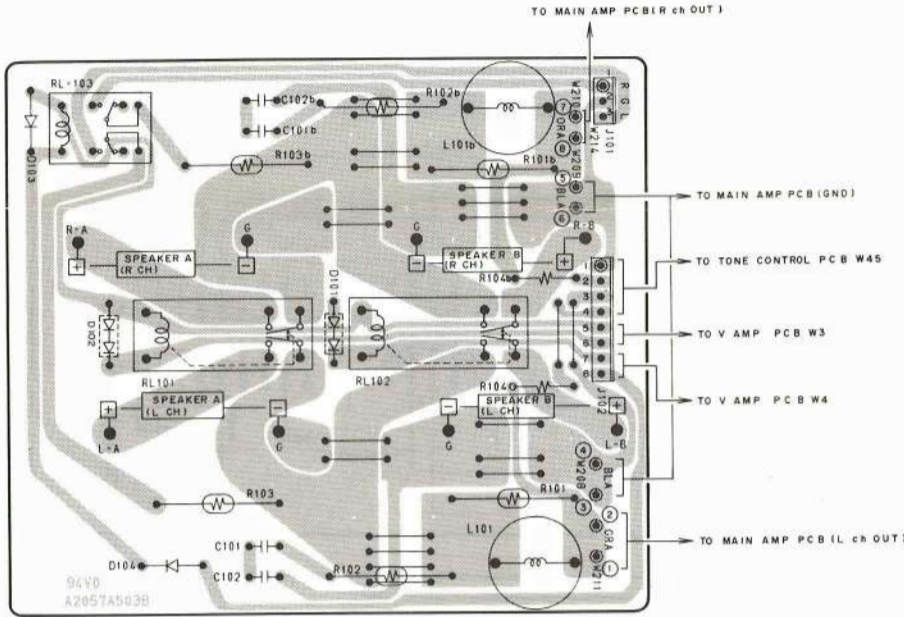
SP TERMINAL PCB A2057A503B
