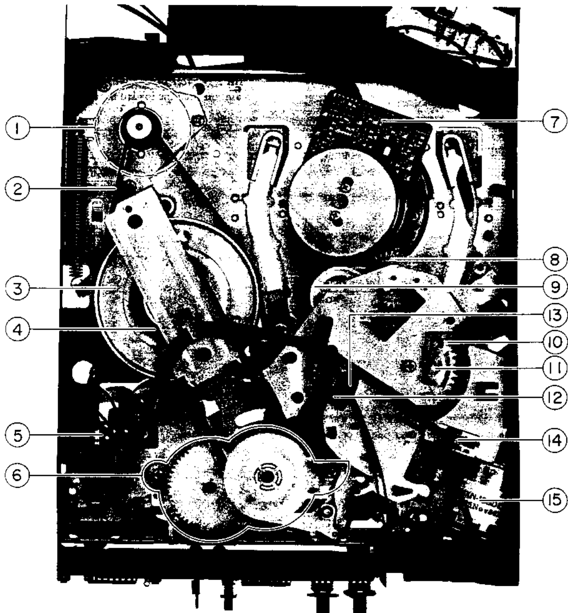
Fig. 5-2 Bottom View
