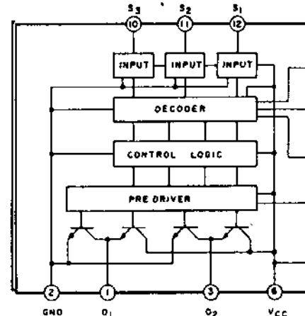
M54548L (CAPSTAN DRIVE IC)
