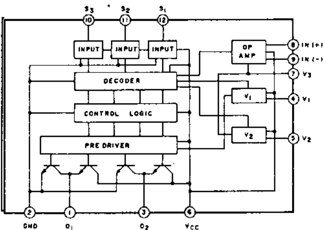
M54548L (CAPSTAN DRIVE IC)
