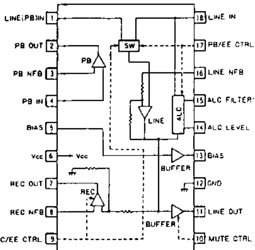
BA5115 (SWITCHLESS REC/PB AMPLIFIER)
