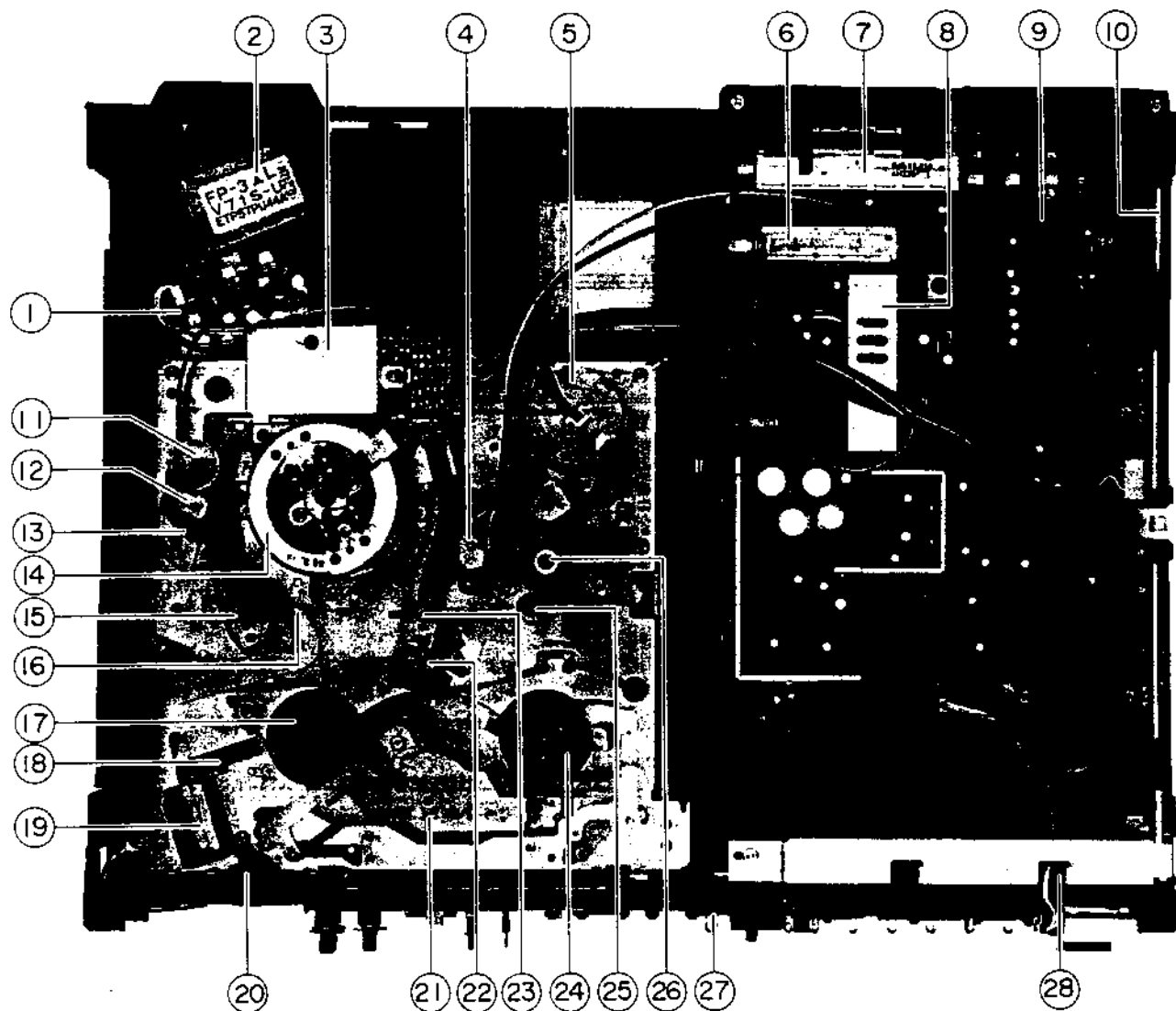
Fig. 5-1 Top View
