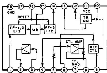
BA5115 (SWITCHLESS REC/PB AMPLIFIER)
