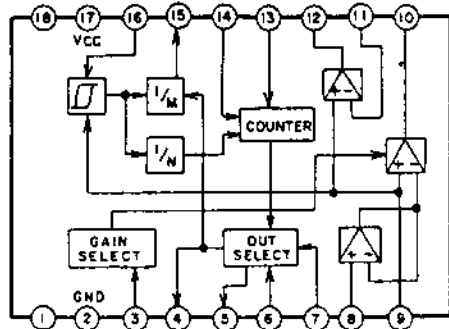
AN3794 (CAPSTAN SERVO INTERFACE IC)
