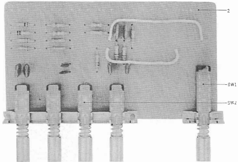
FIG. 7 PHOTO OF SW. P.C. BOARD (A5-5061) BLOCK
