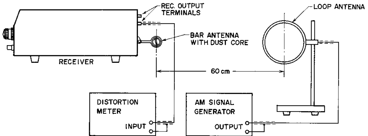
Fig. 16 INSTRUMENT CONNECTIONS
