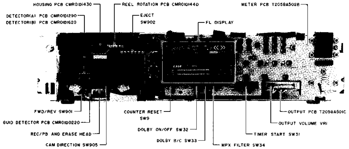
Fig. 4-1 Front View
