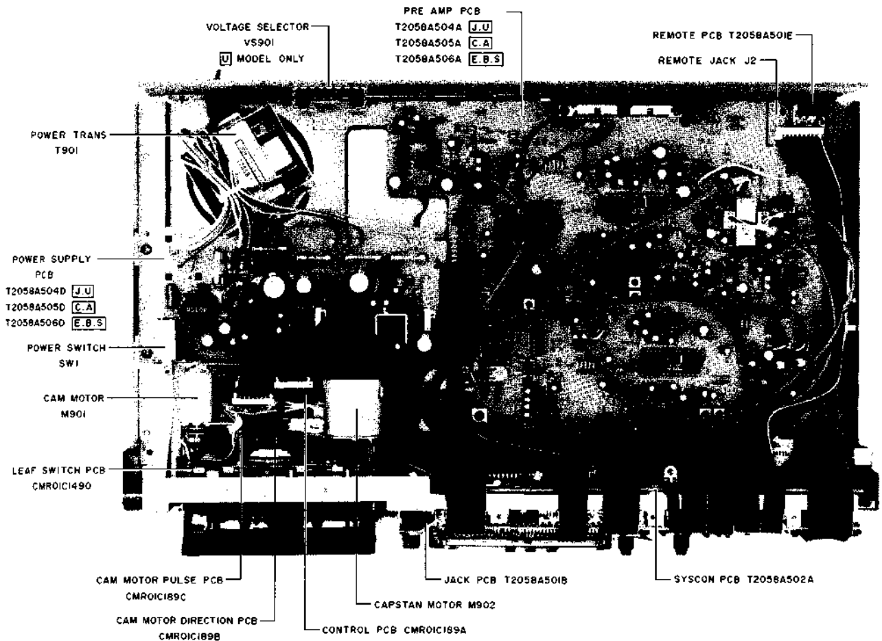
Fig. 4-2 Top View
