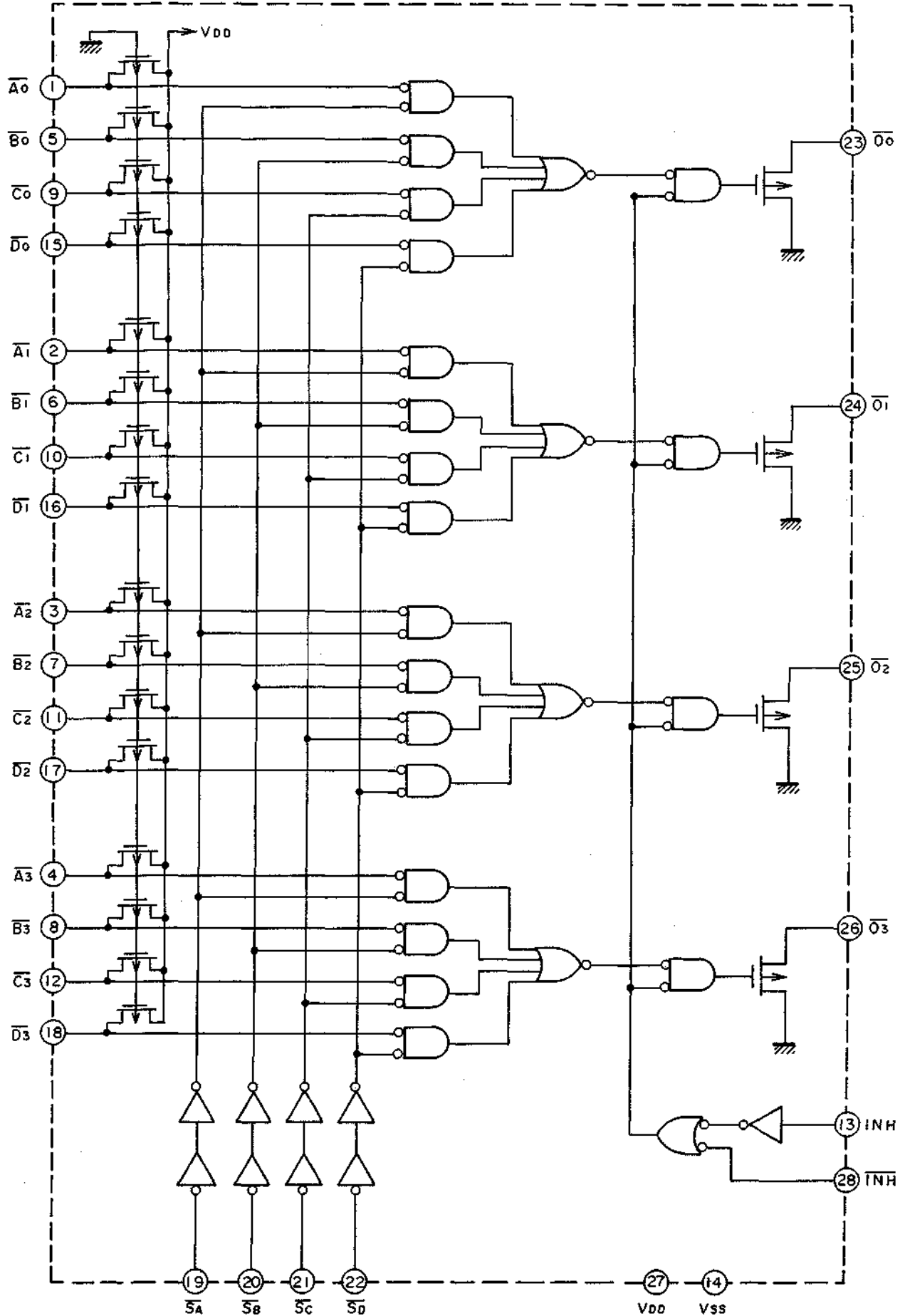
SCHEMATIC DIAGRAM GX-7
