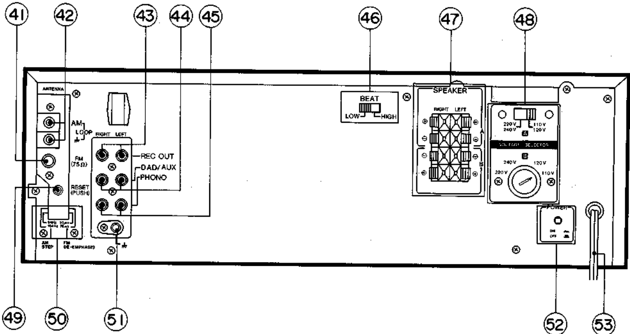
Fig. 3-4 Rear View
