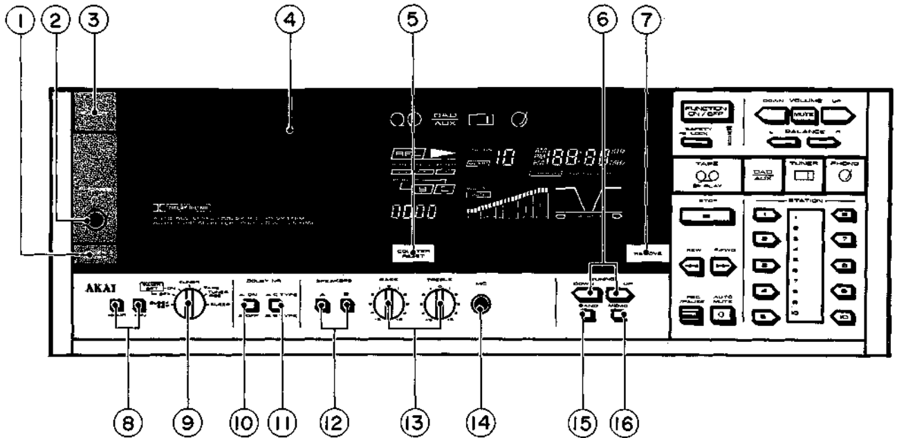
Fig. 3-1 Front View
