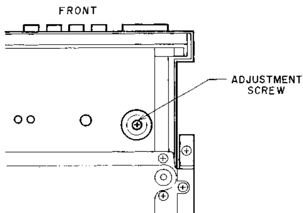
Fig. 5-2 Adjustment Point
