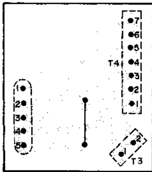
TERMINAL PCB 22193662
