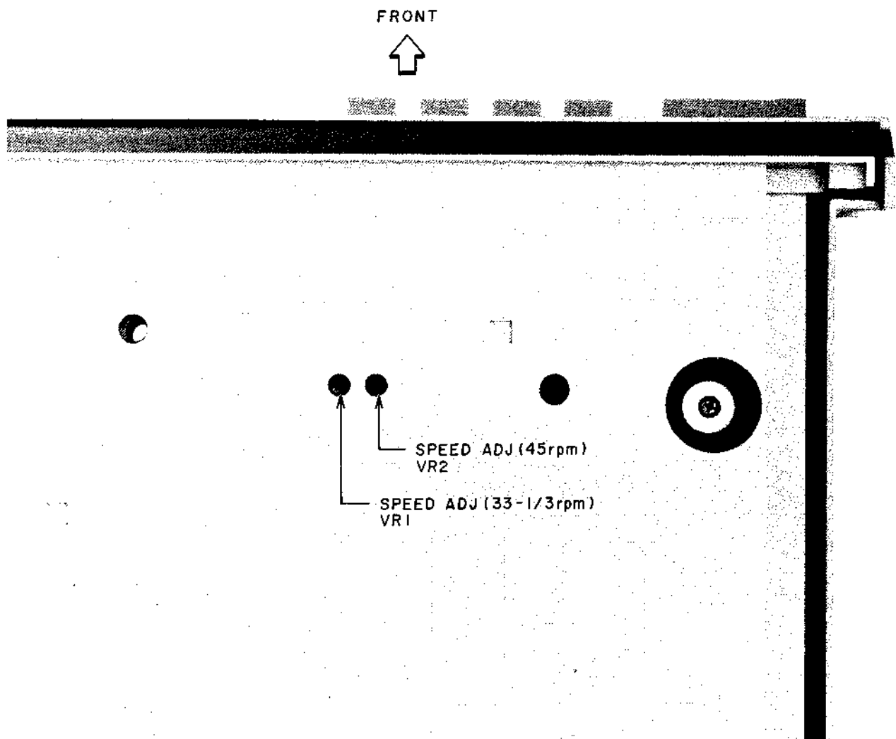
Fig. 5-6 Adjustment Point
