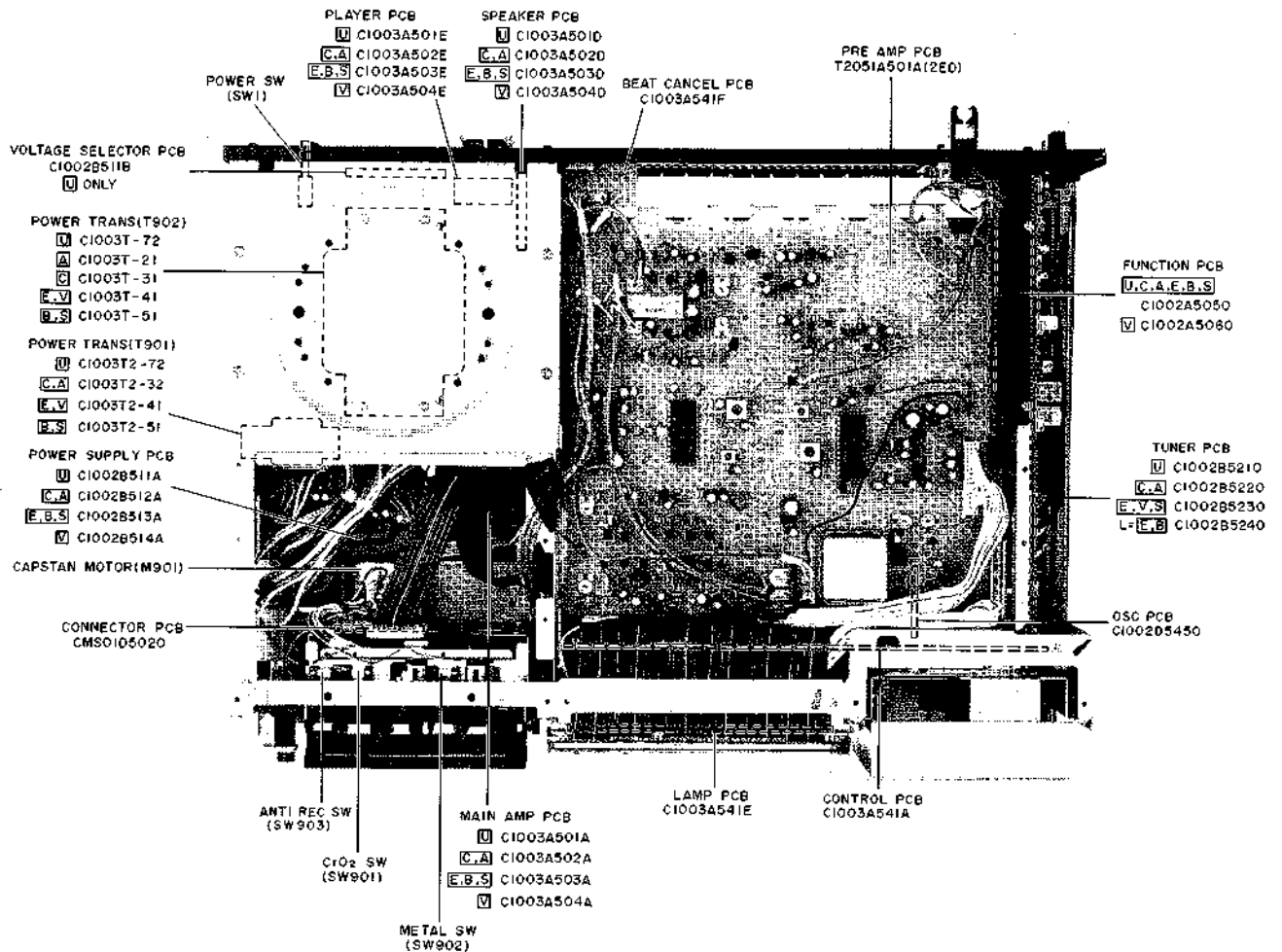
Fig. 4-2 Top View
