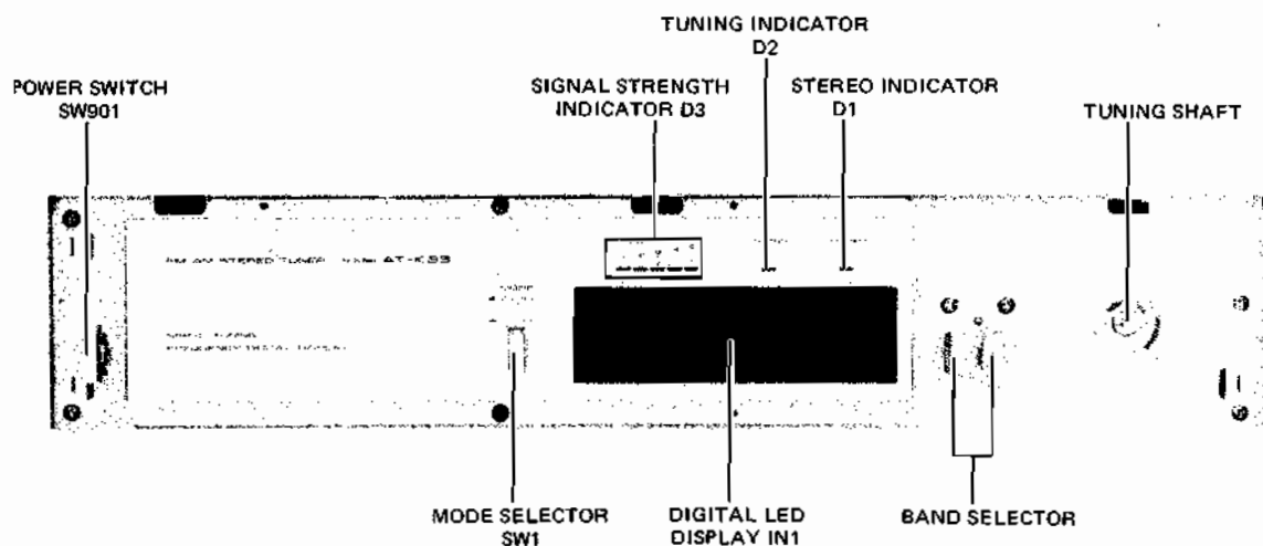
Fig. 2 Front View
