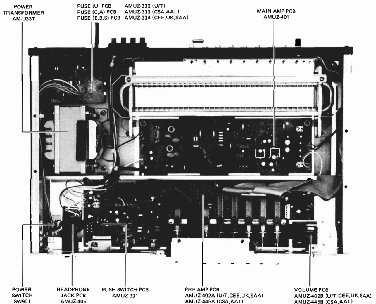
Fig. 3 Top View
