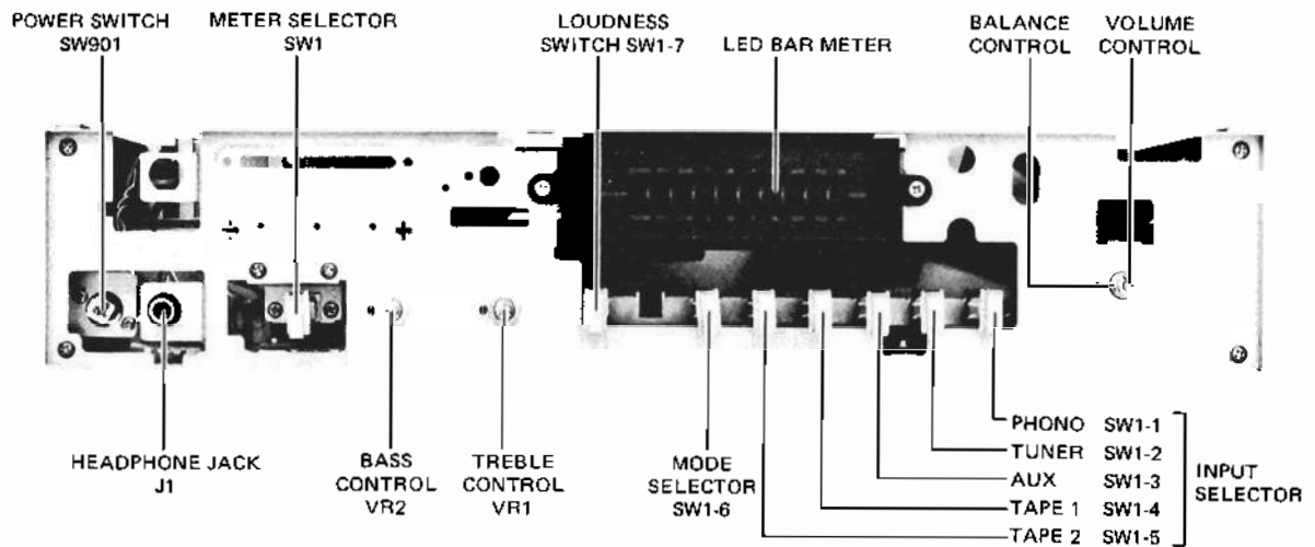
Fig. 2 Front View
