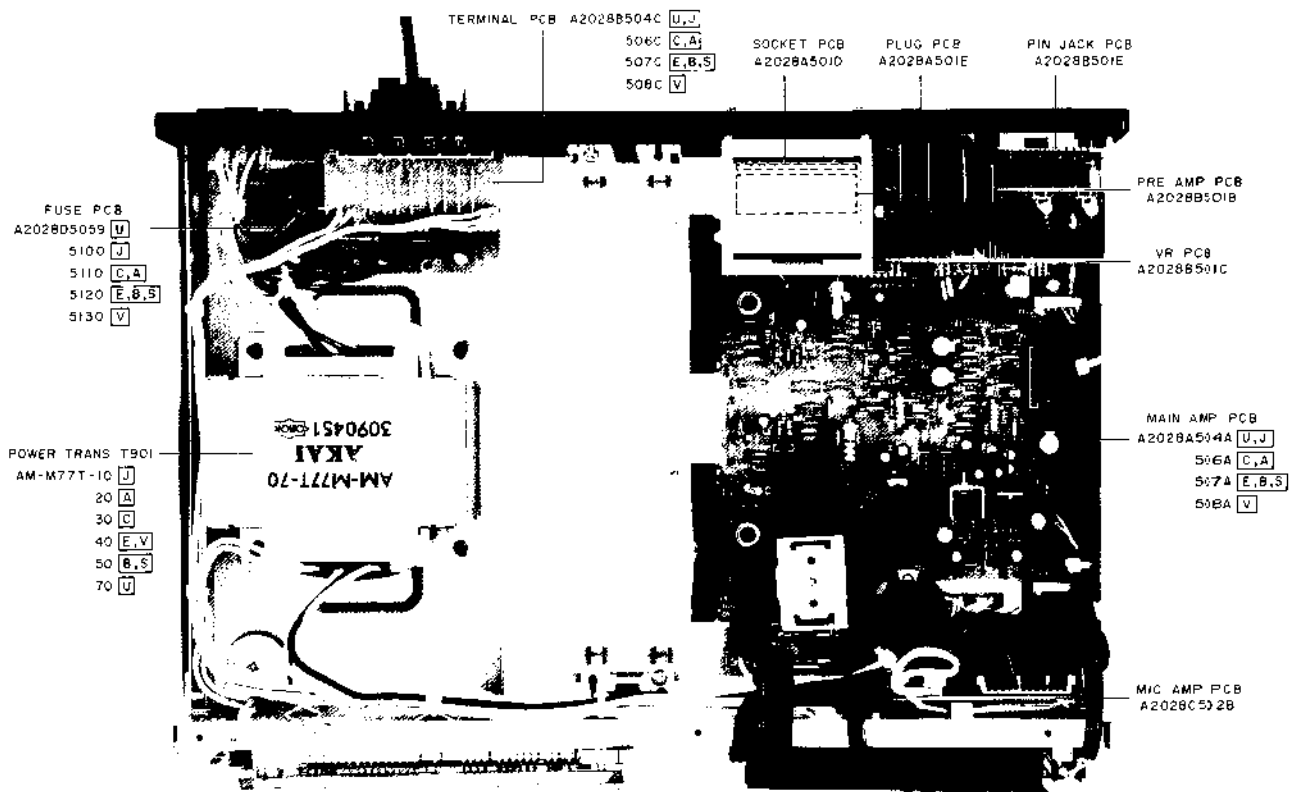
Fig. 4-2 Upper View
