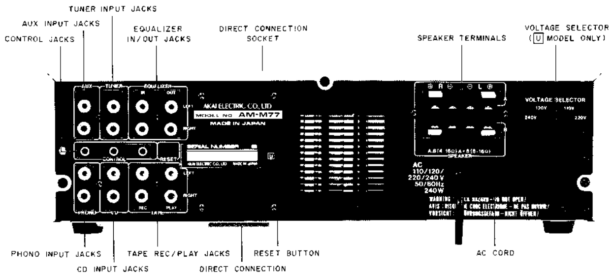
Fig. 3-2 Rear View
