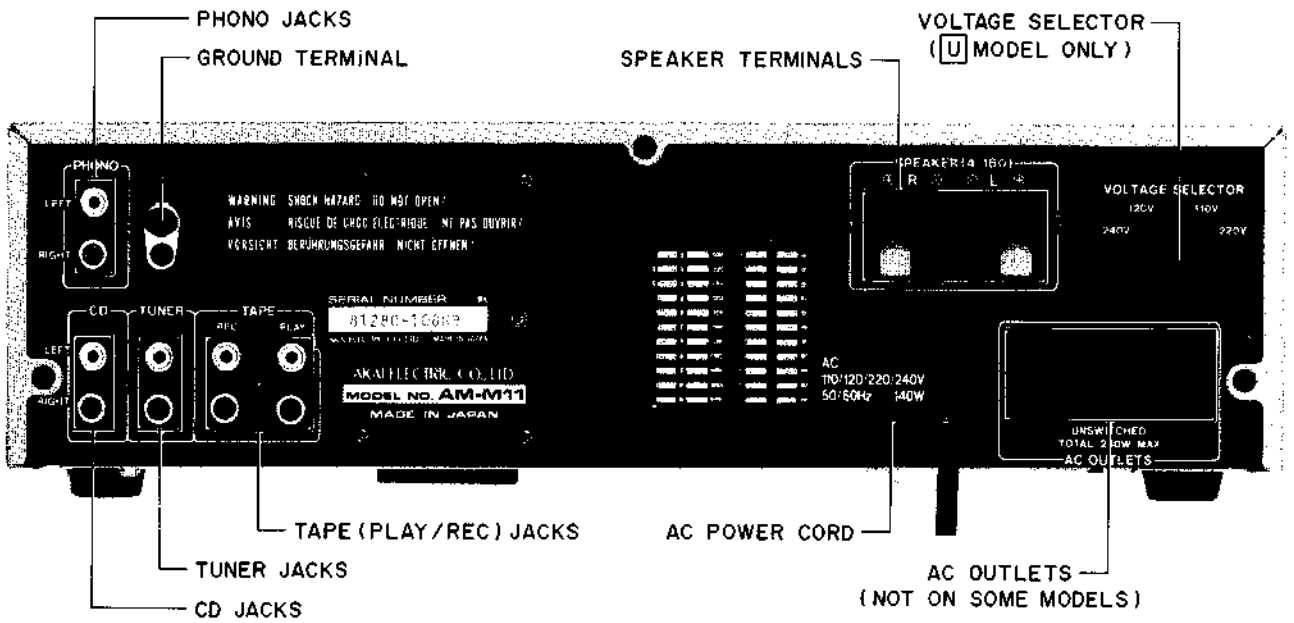
Fig. 3-2 Rear View
