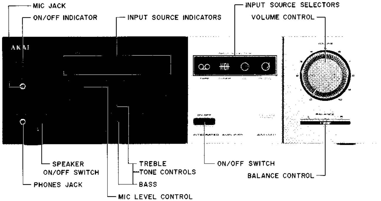
Fig. 3-1 Front View
