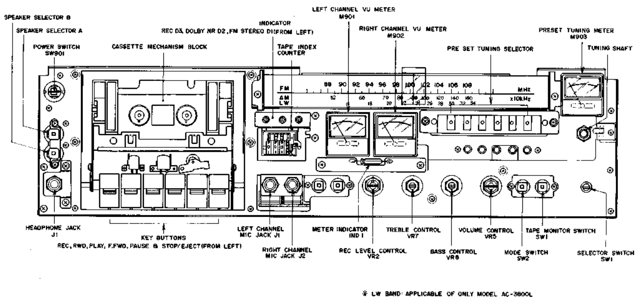
Fig. 6 Front View
