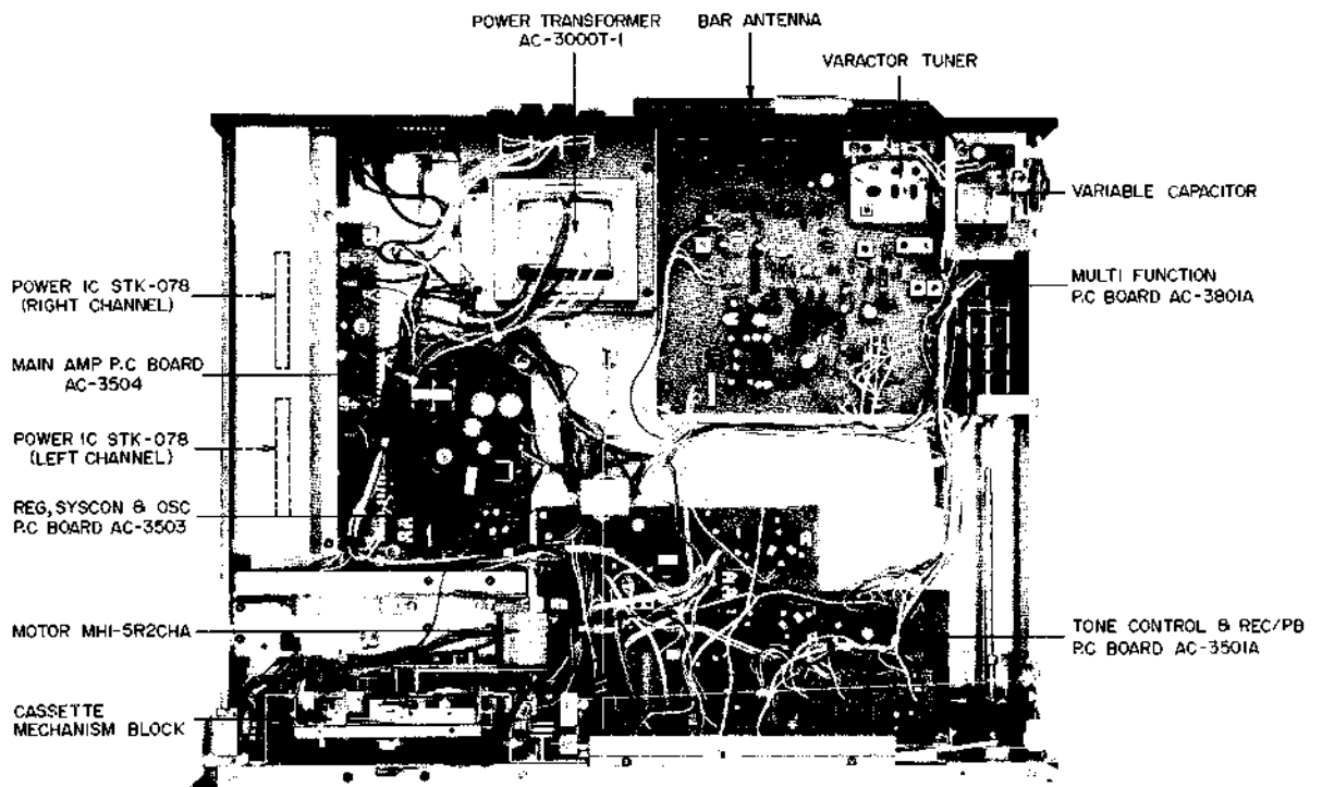
Fig. 8 Top View of Model AC-3800L
