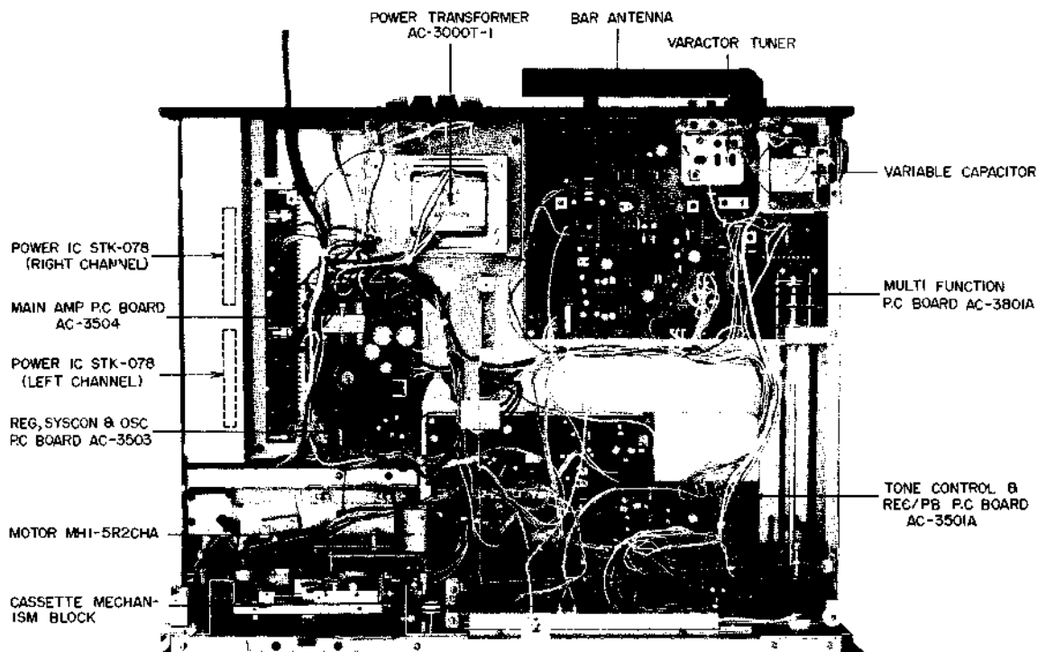
Fig. 7 Top View of Model AC-3800
