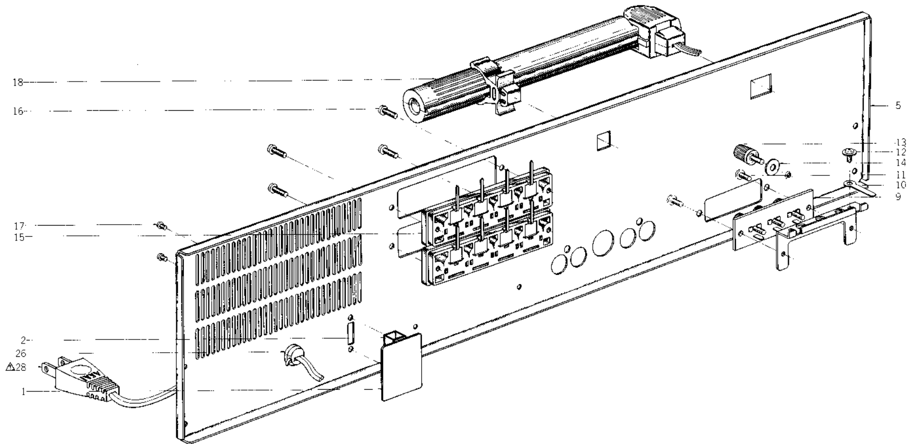
12. ILLUSTRATION OF REAR PANEL BLOCK (AC-3800)
