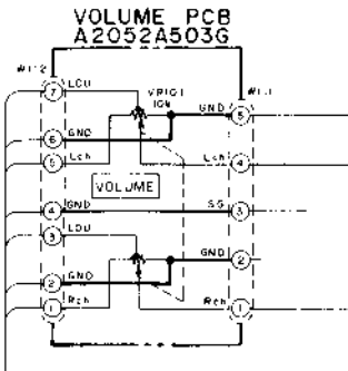
VOLUME PCB A2052A503G
