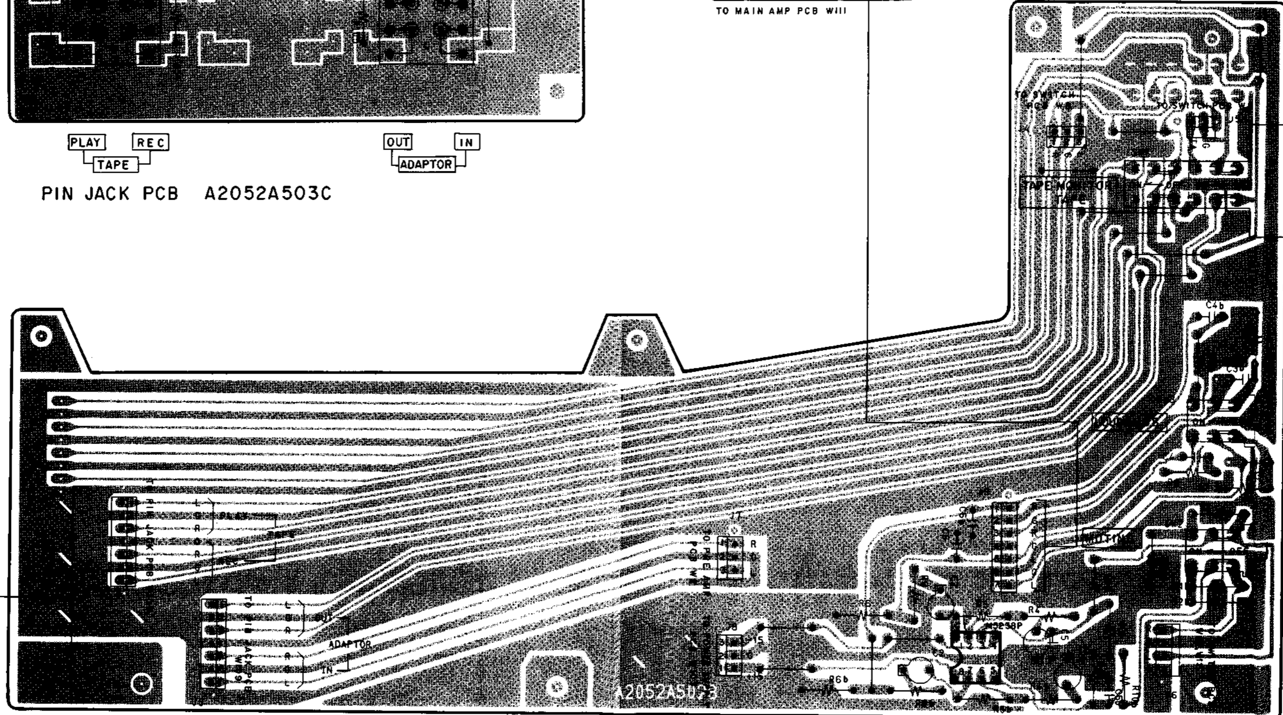
TAPE SELECTOR PCB A2052A502B
