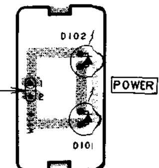
POWER LED PCB A2052A503K
