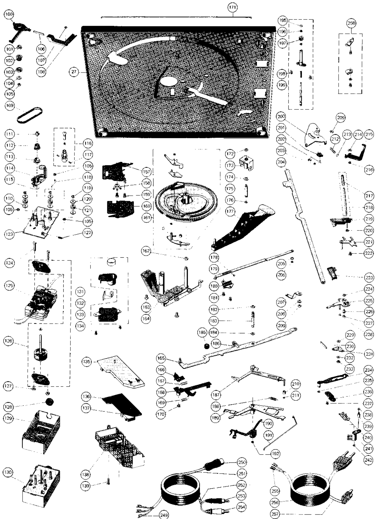
Fig. 21 Exploded view 2
