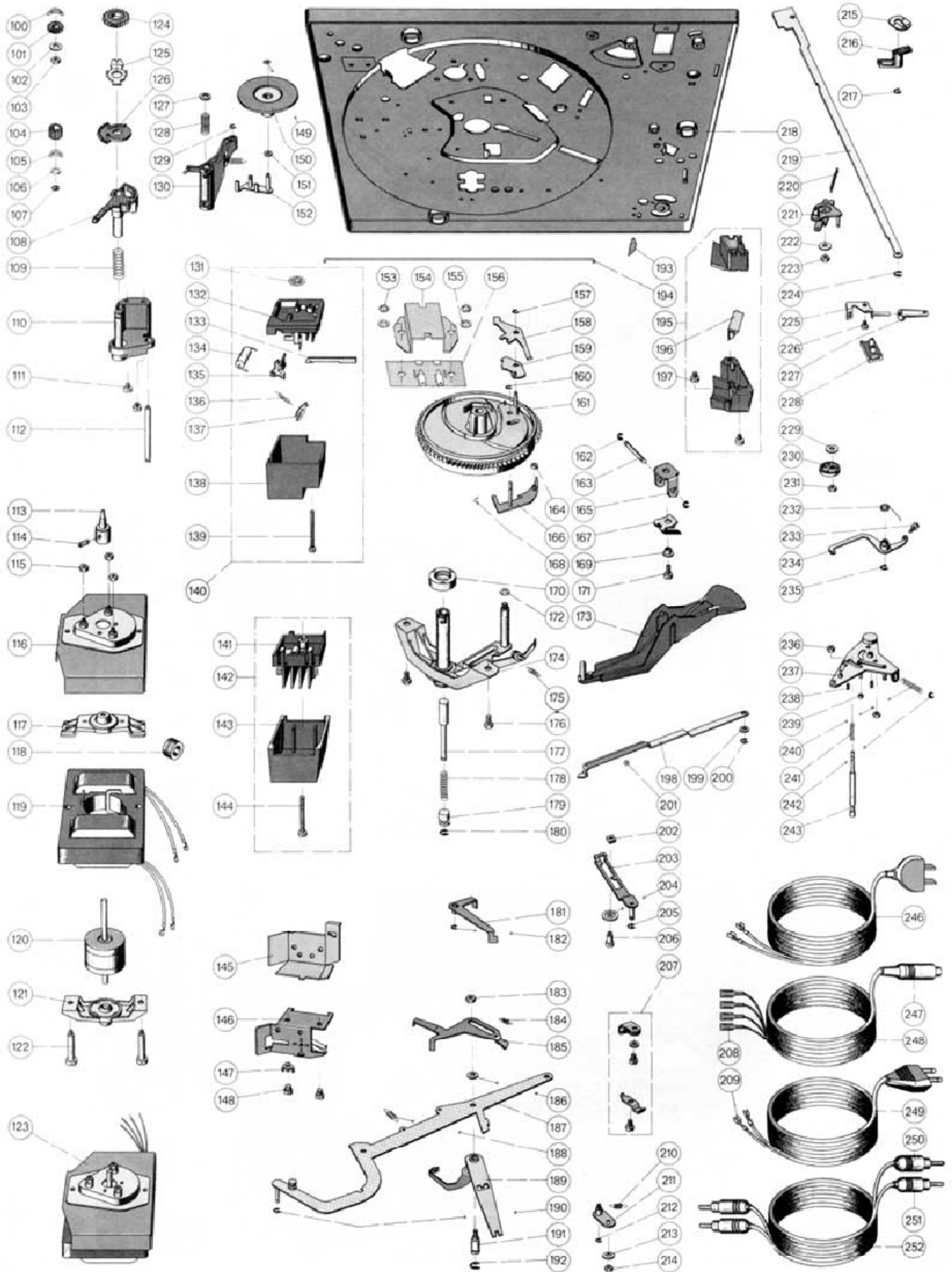
Fig. 29 Exploded view, parts below chassis
