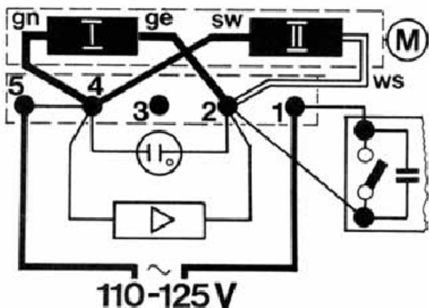
Fig. 3 Motor field connections (with voltage selector)
