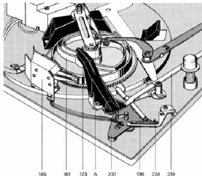
Fig. 12 Tonearm guide mechanism
