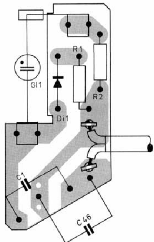
Fig. 6 Circuit board (output stages)
