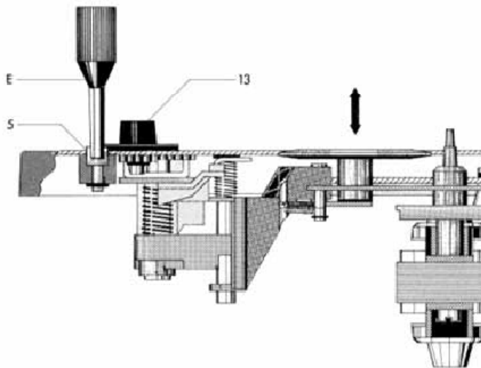
Fig. 7 Position of idler wheel
