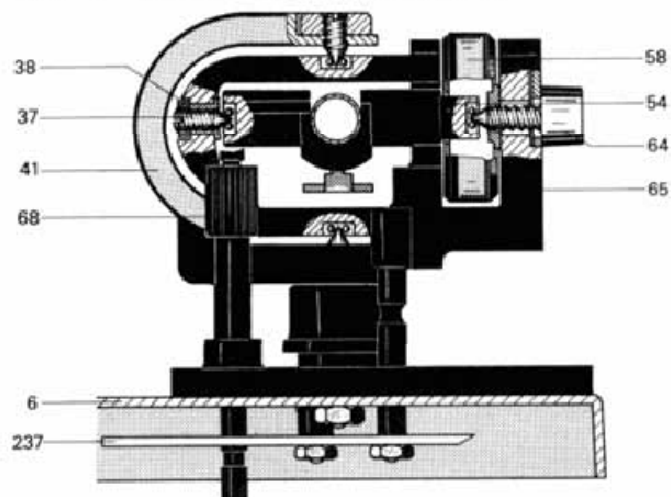
Fig. 9 Tonearm bearing assembly
