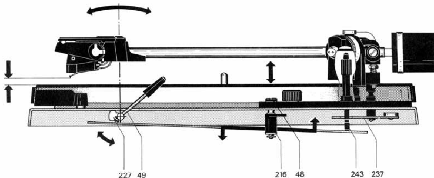
Fig. 13 Tonearm lift (tonearm raised)
