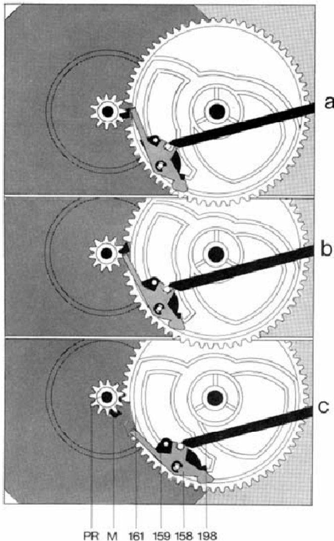
Fig. 18 Actuating "change" or "shut-off"
