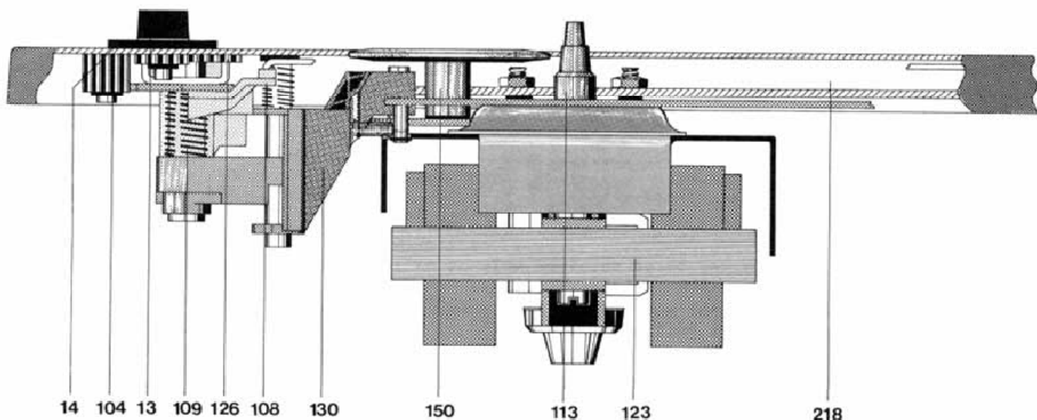
Fig. 2 Motor suspension and platter drive
