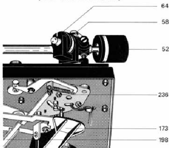
Fig. 10 Tonearm bearing assembly (view from underneath)
