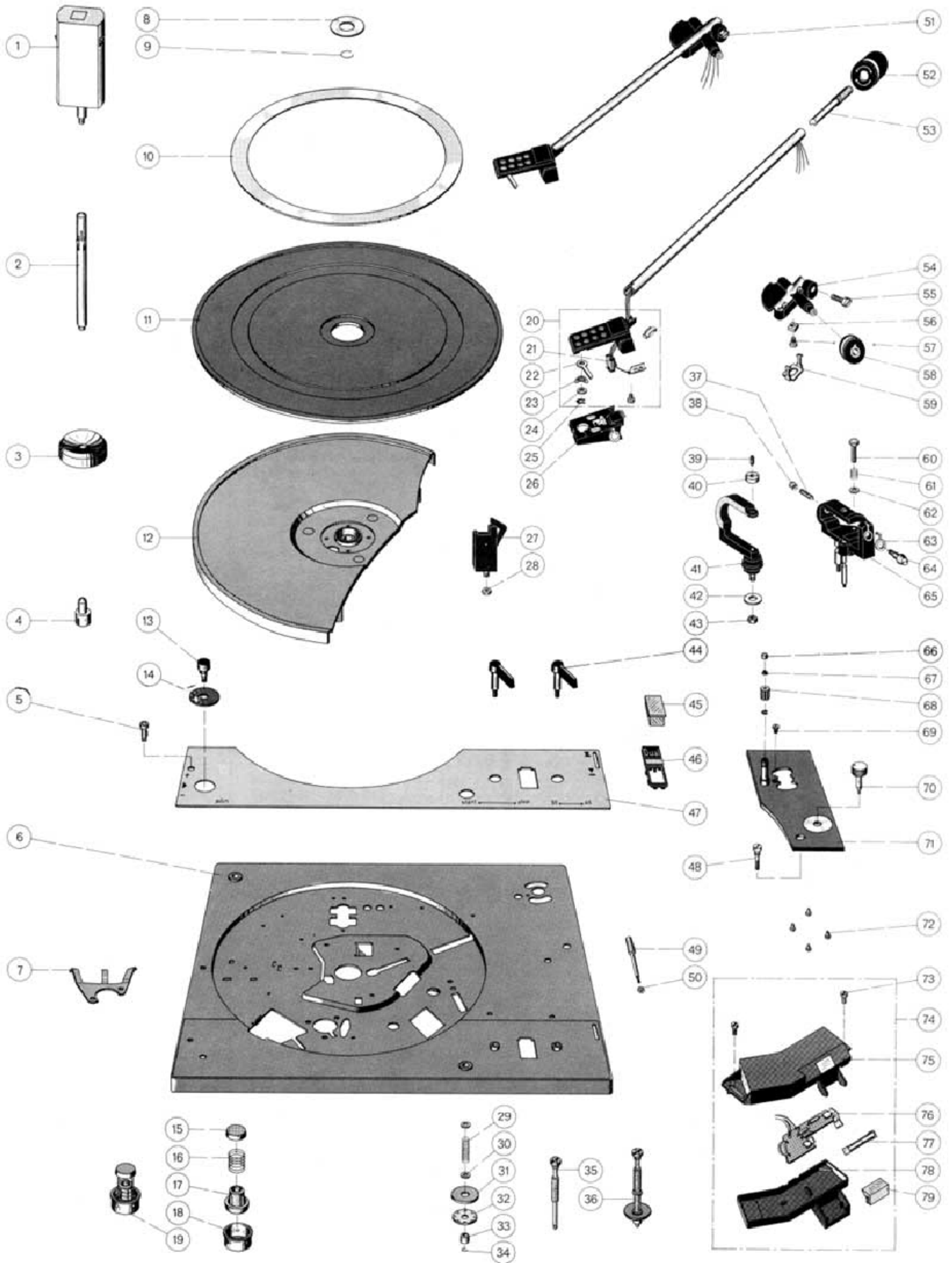
Fig. 28 Exploded view, parts above chassis
