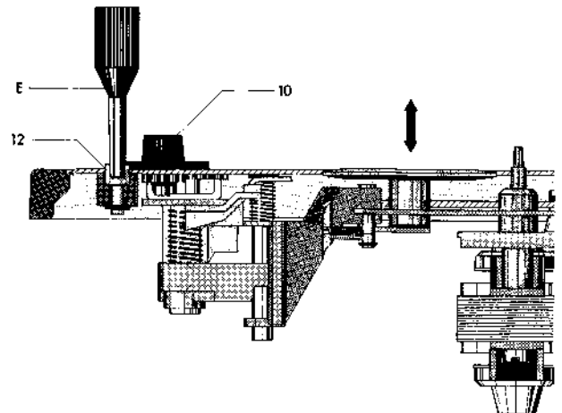
Fig. 4 Position of idler wheel
