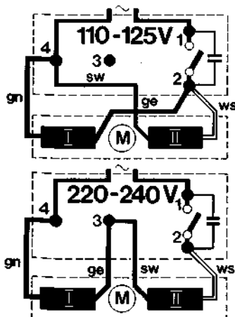
Fig. 5 Motor field connections (less voltage selector)
