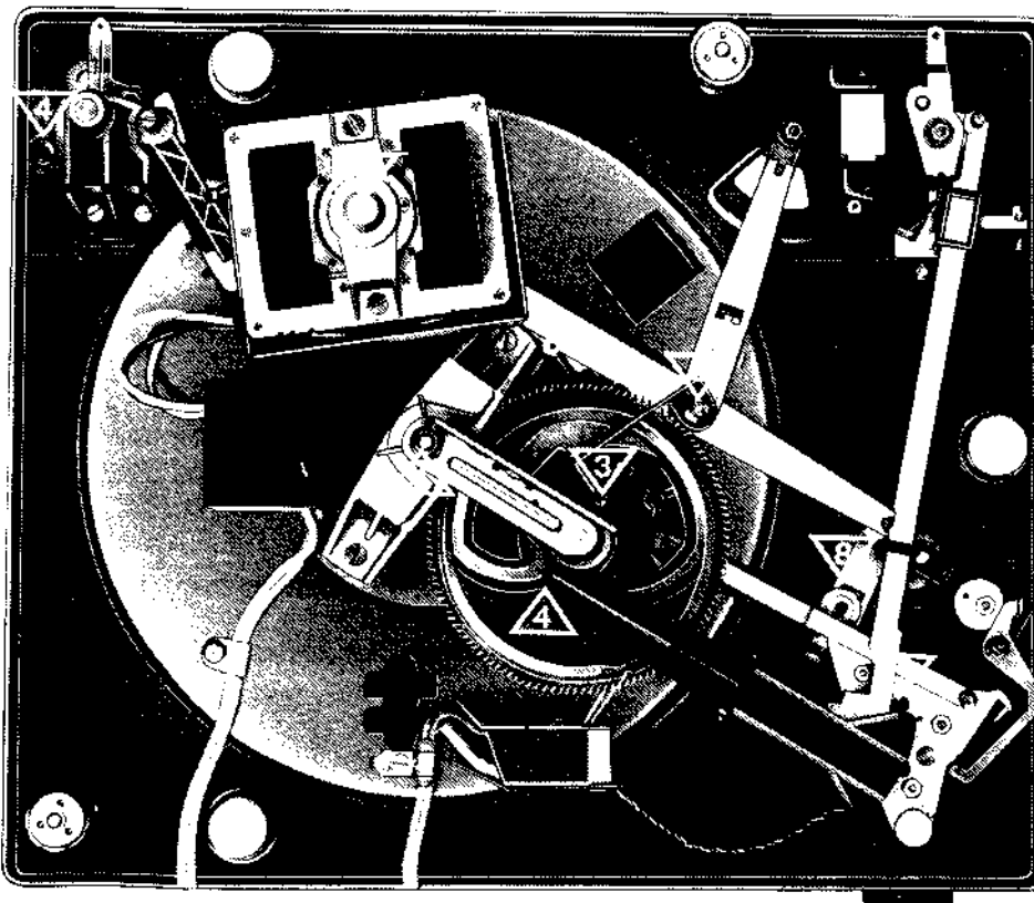
Fig. 27 Lubrication points below chassis
