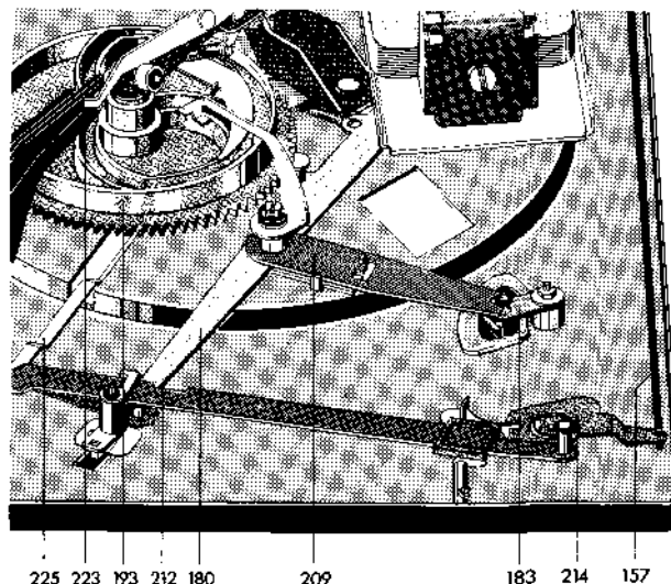
Fig. 13 Start position
