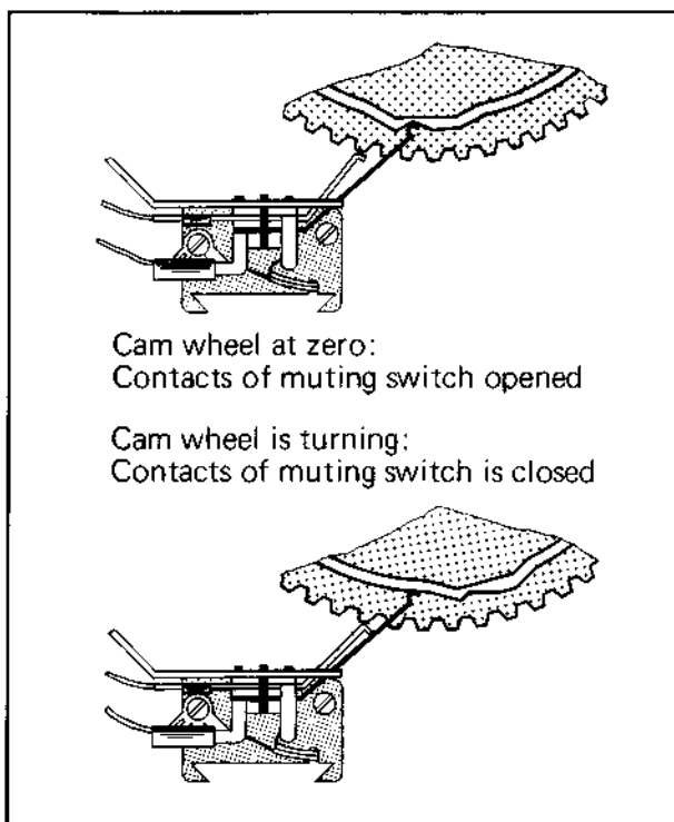
Fig. 15 Muting Switch
