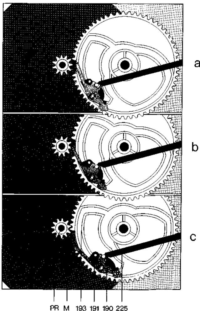
Fig. 17 Actuating "change" or "shut-off"
