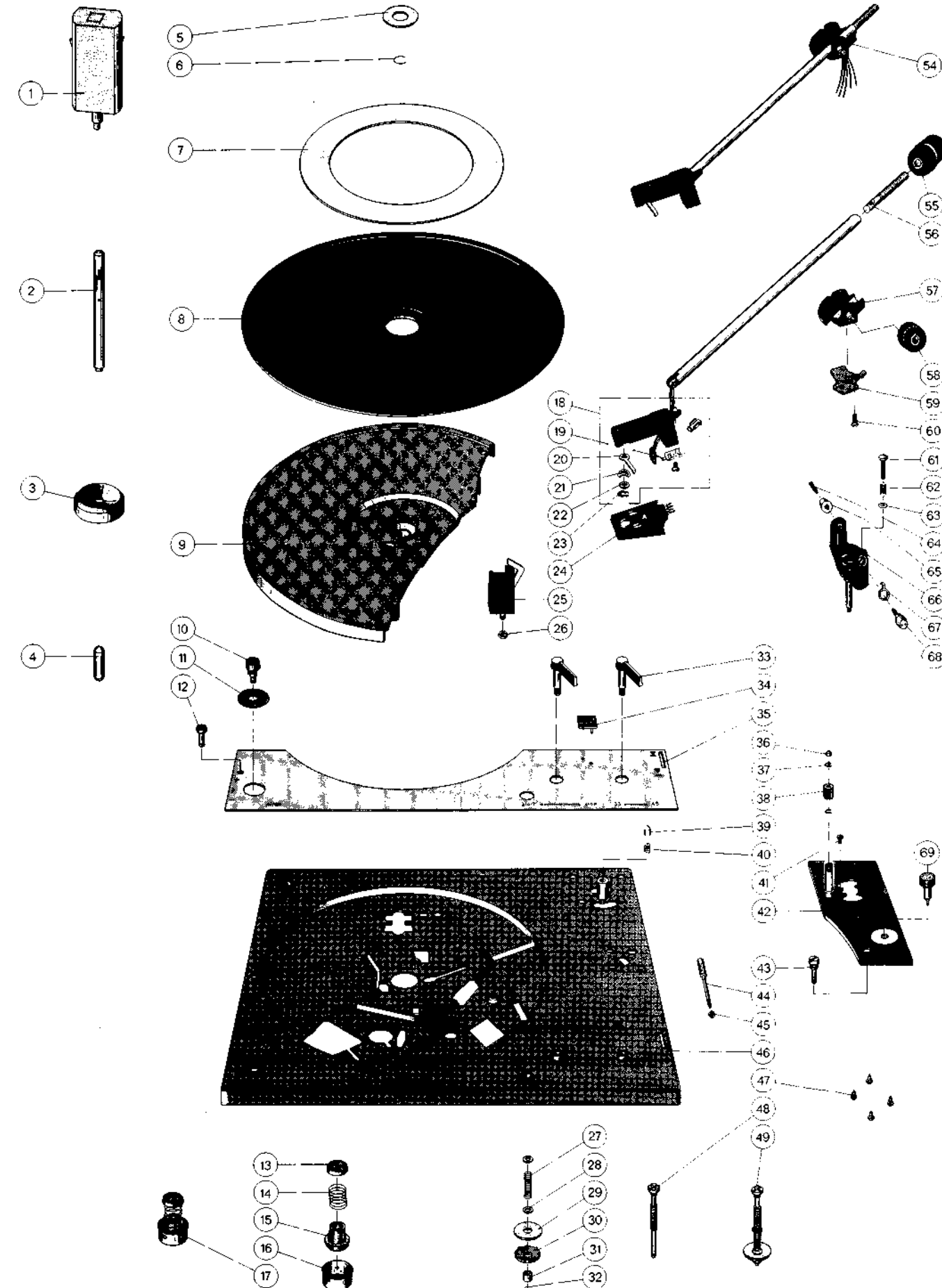
Fig. 24 Exploded view, above chassis
