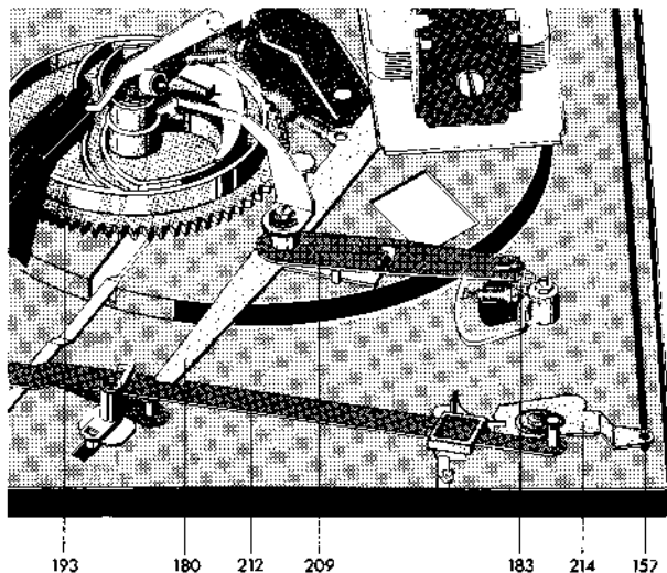
Fig. 14 Stop position
