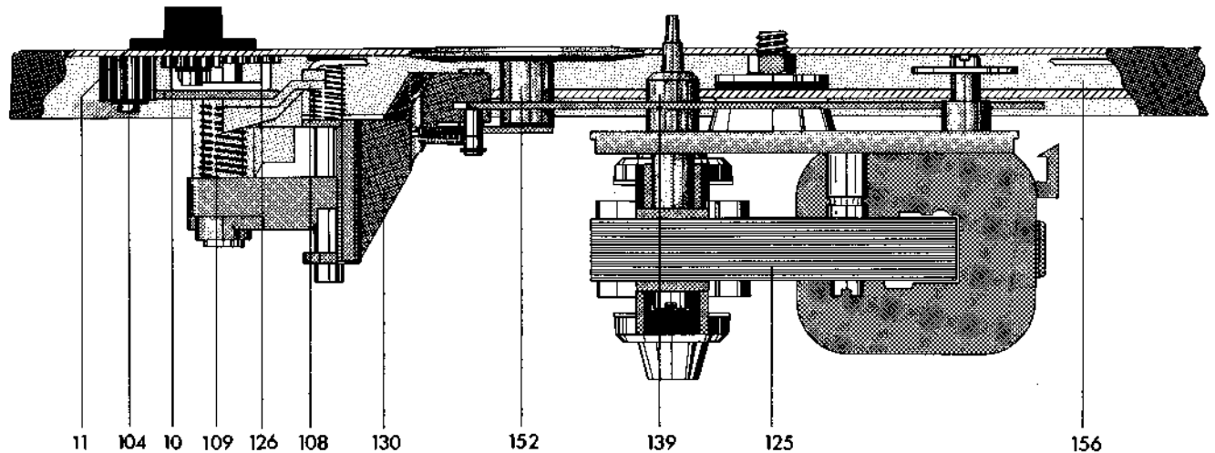
Fig. 3 Motor suspension and platter drive Dual 1225
