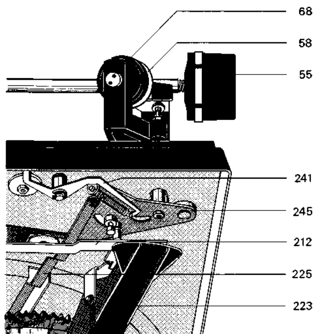
Fig. 8 Tonearm bearing assembly (view from underneath)
