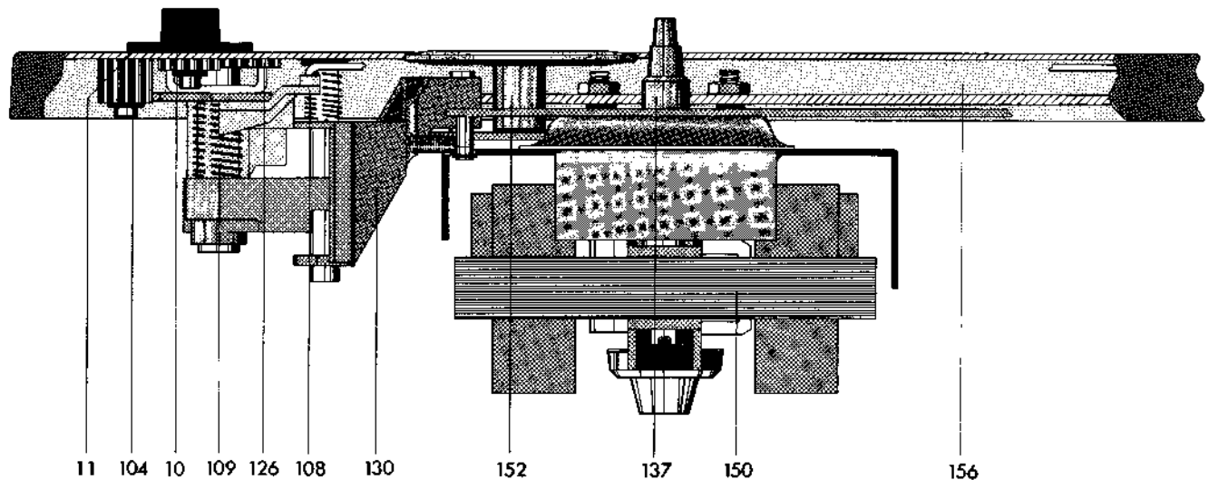
Fig. 3 Motor suspension and platter drive Dual 1225
