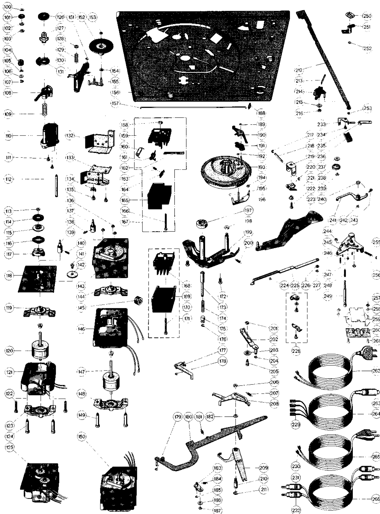
Fig. 25 Exploded view, below chassis
