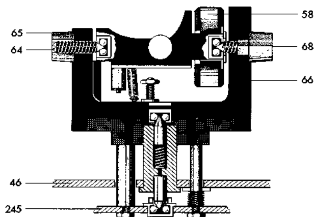
Fig. 7 Tonearm bearing assembly
