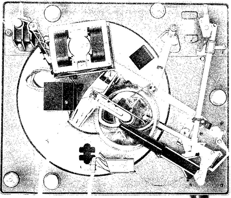
Fig. 30. Lubrication points below chassis
