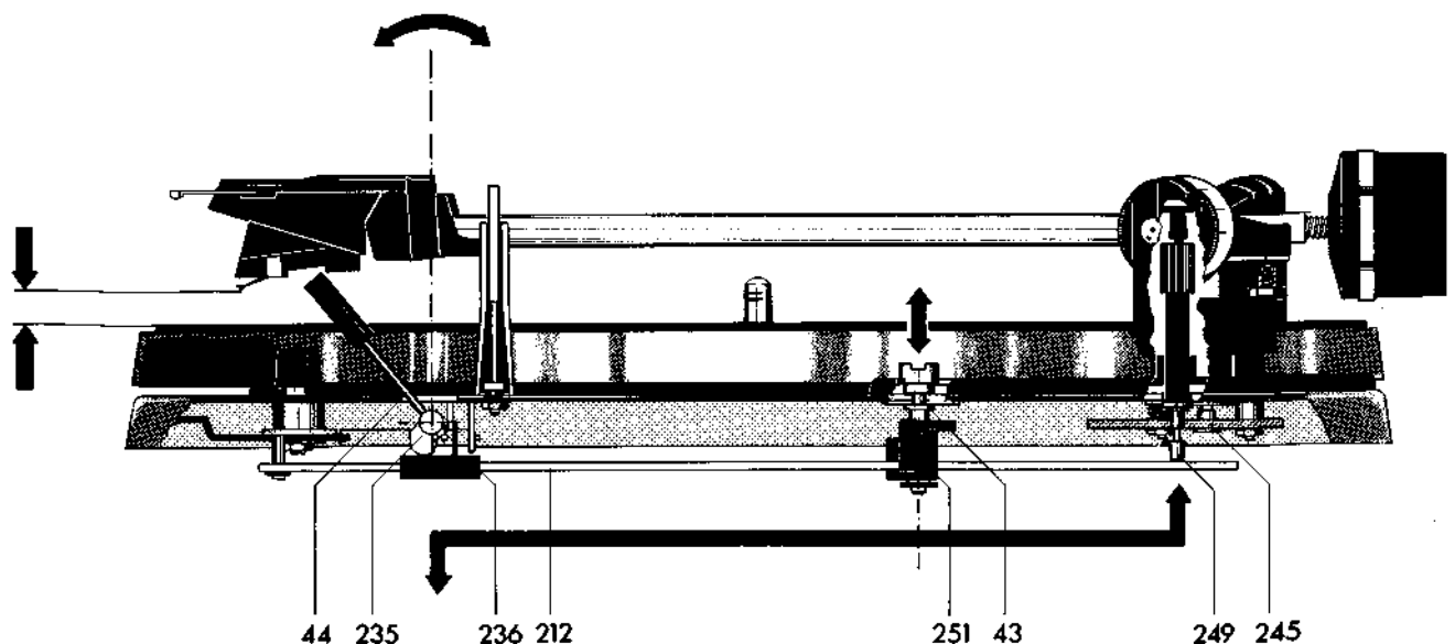
Fig. 12 Tonearm lift (tonearm raised)
