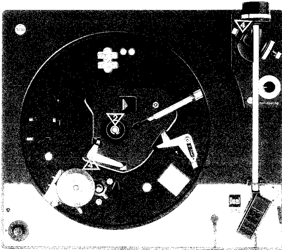
Fig. 29. Lubrication points above chassis
