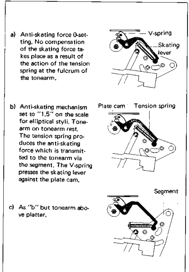
Fig. 9 Anti-skating force
