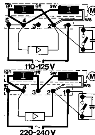
Fig. 6 Motor field connections (with voltage selector)
