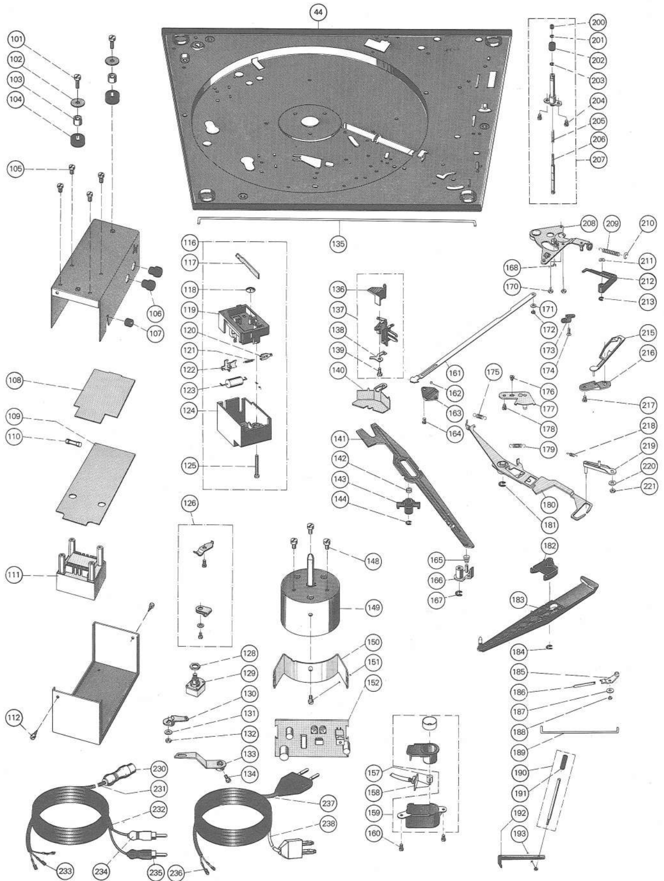
Fig. 19 Exploded view 1
