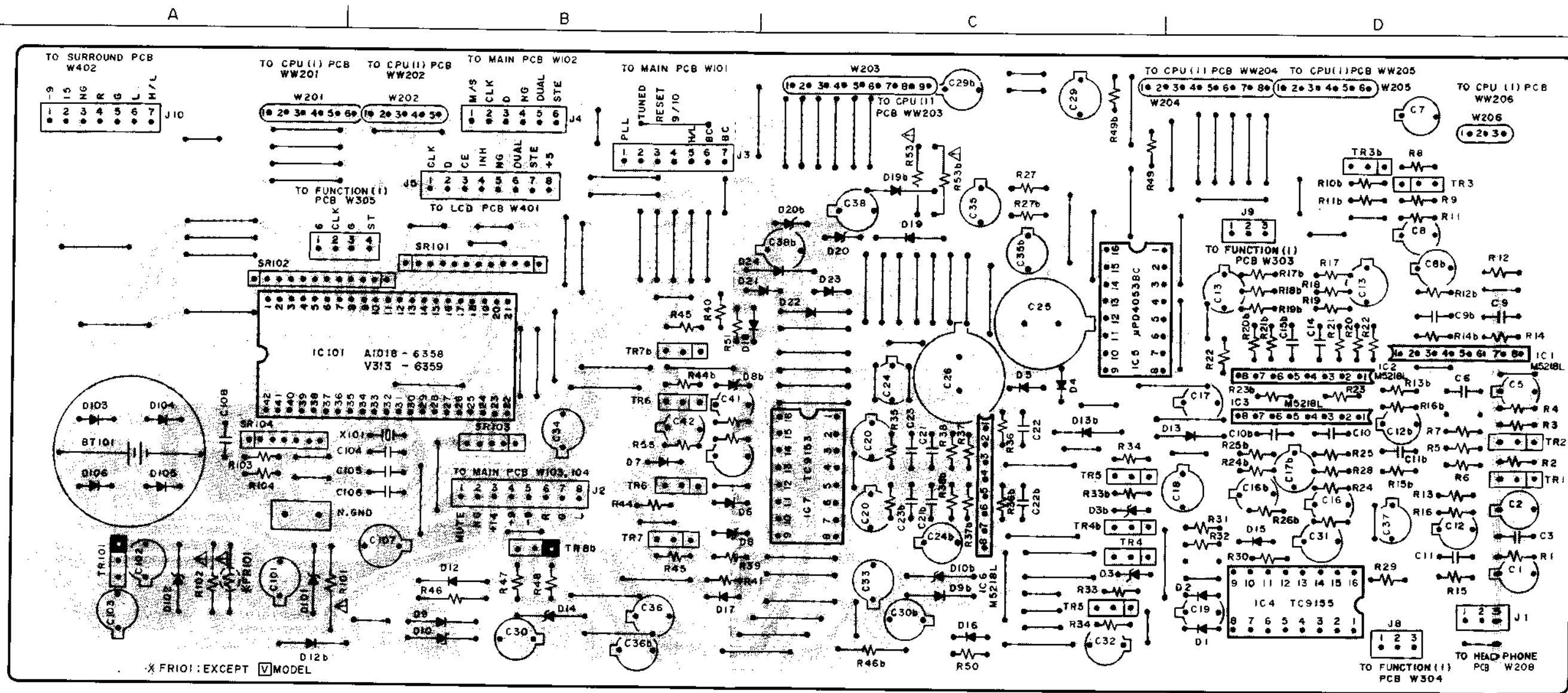
CPU(2) PCB A1018A507B
