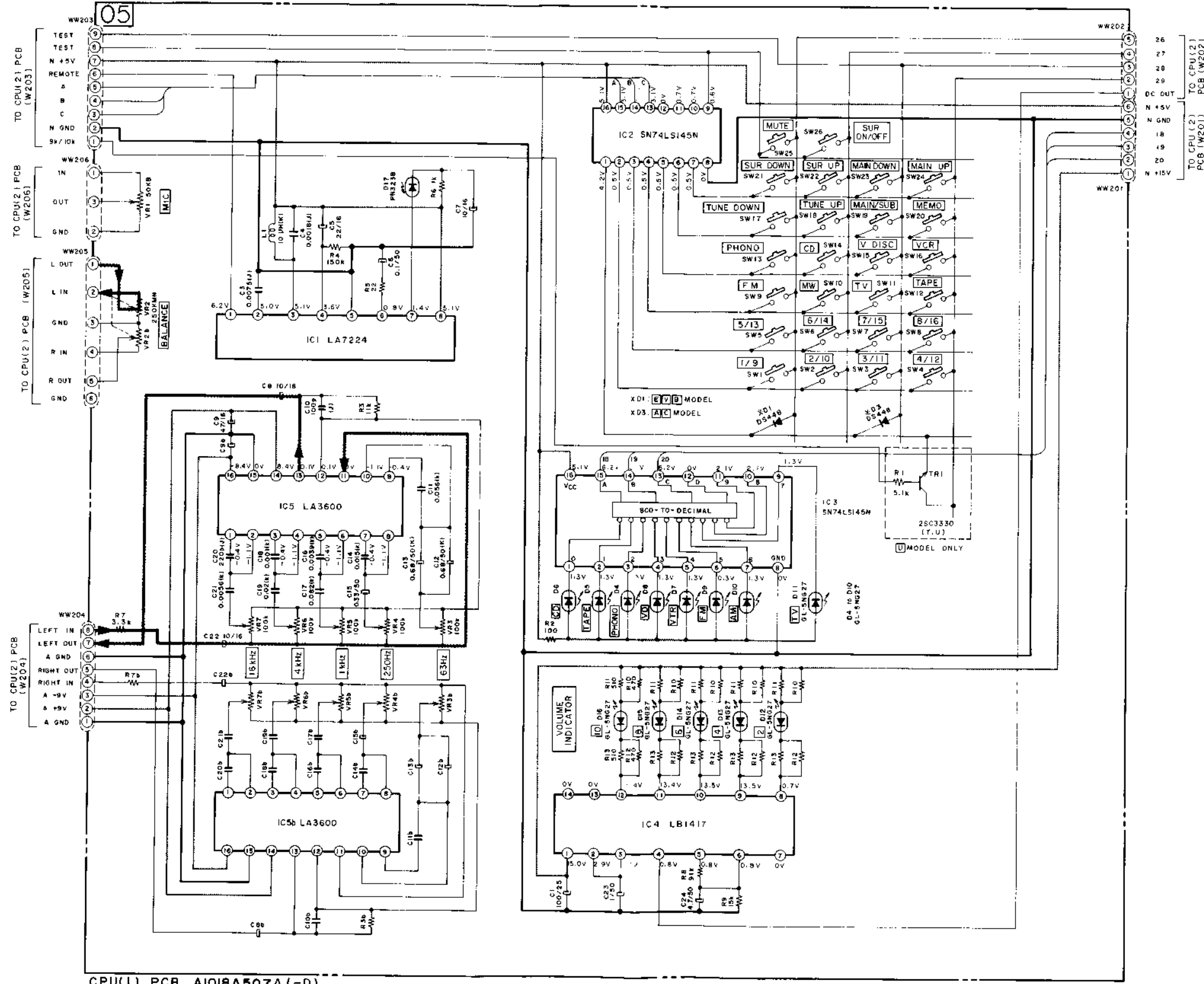
CPU(1) PCB A1018A507A (-D)
