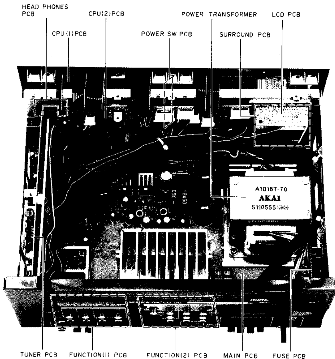
Fig. 3-1 Top View
