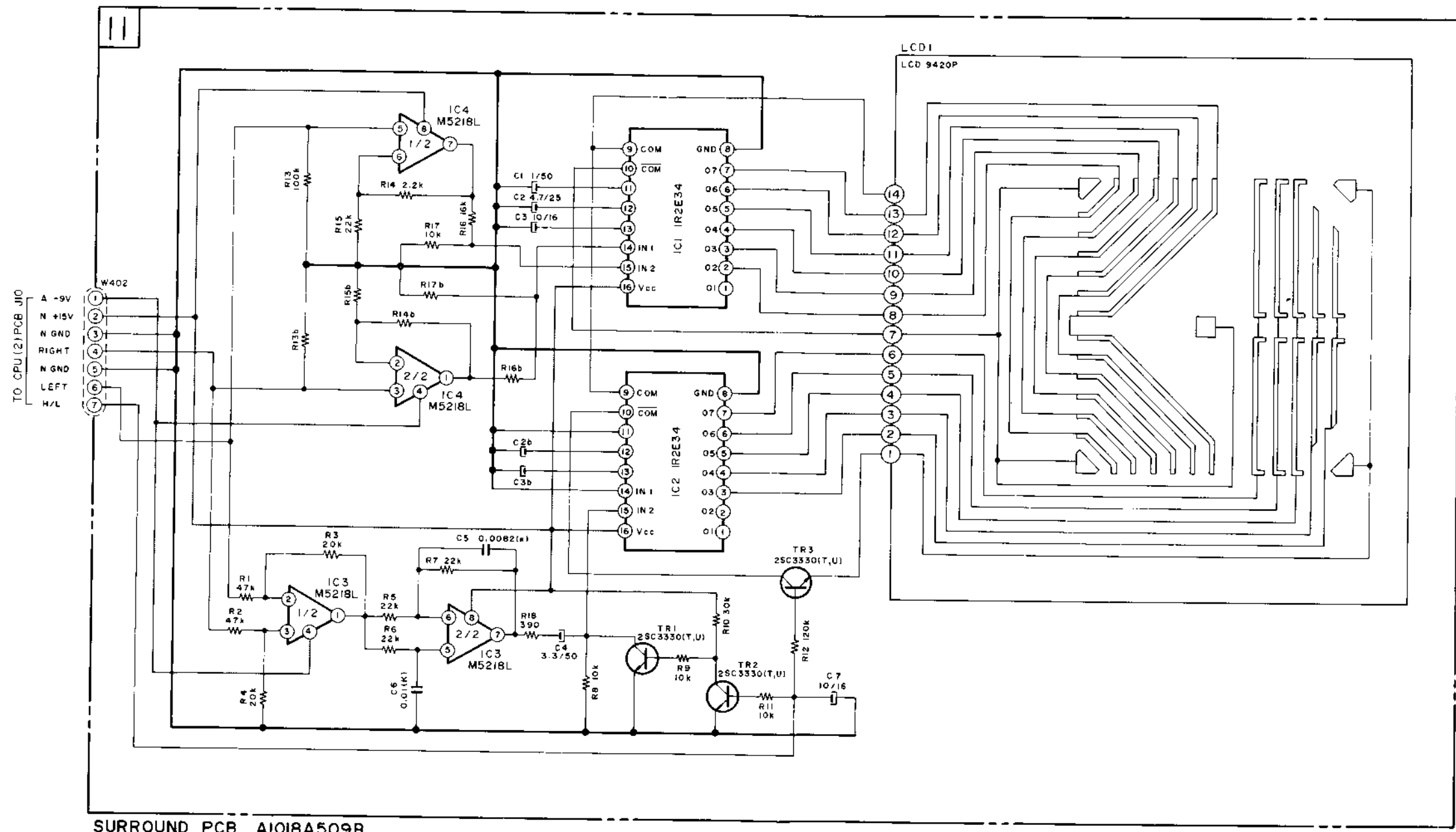
SURROUND PCB A1018A509B
