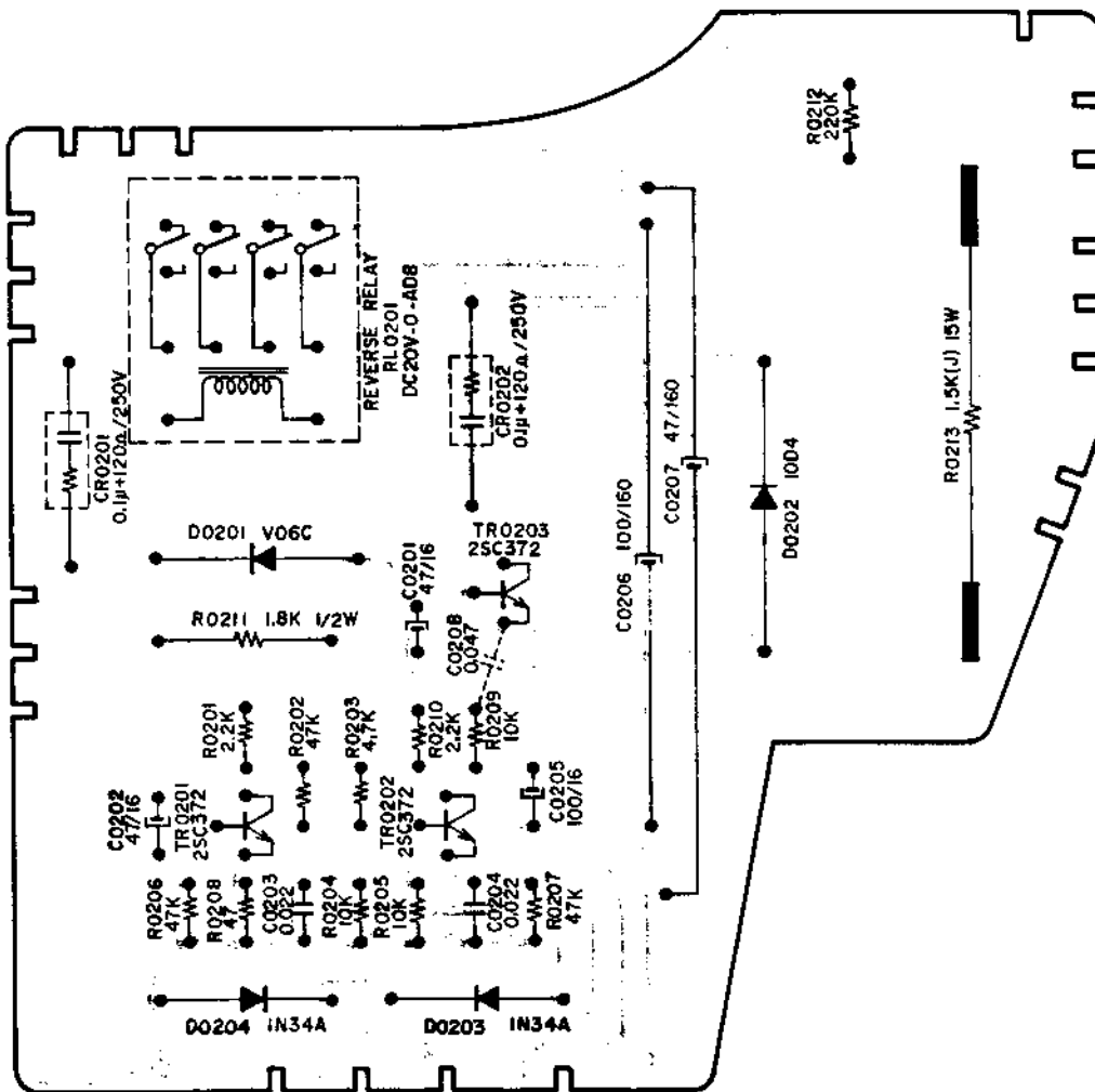
SYSTEM CONTROL P.C. BOARD (MR-504)
