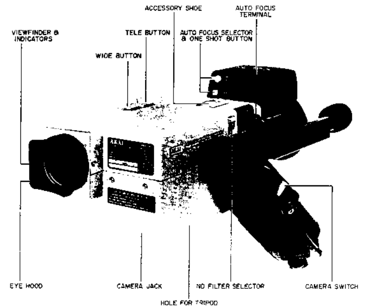
Fig. 1 Controls
