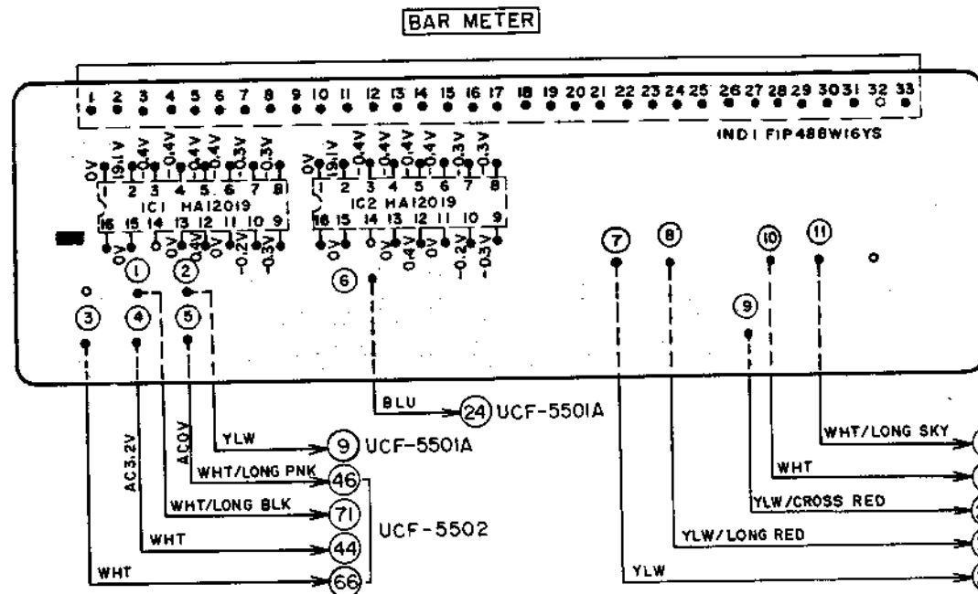
Meter P.C Board CE-5209
