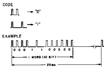
TRANSMISSION CODE (M50110P PIN ⑩)
