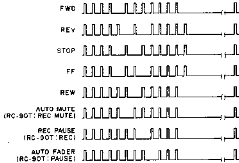
WAVE FORM OF LSI M50110P PIN ⑫ (RC-90T/RC-91T)
