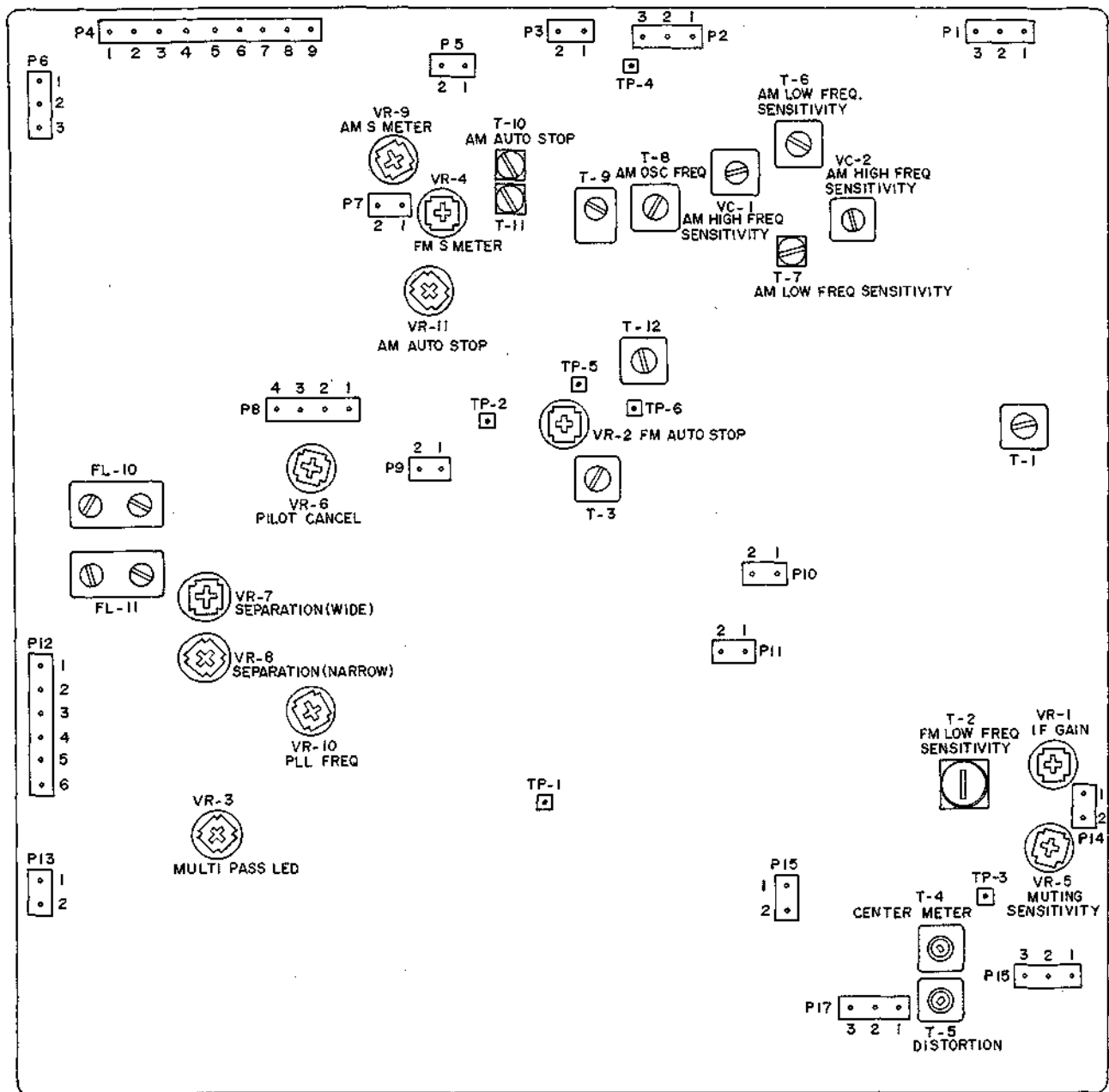
Fig. 7-4 Tuner P.C Board (PT-2001)
