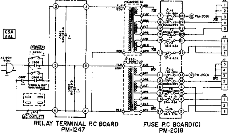
RELAY TERMINAL P.C. BOARD PM-1247
