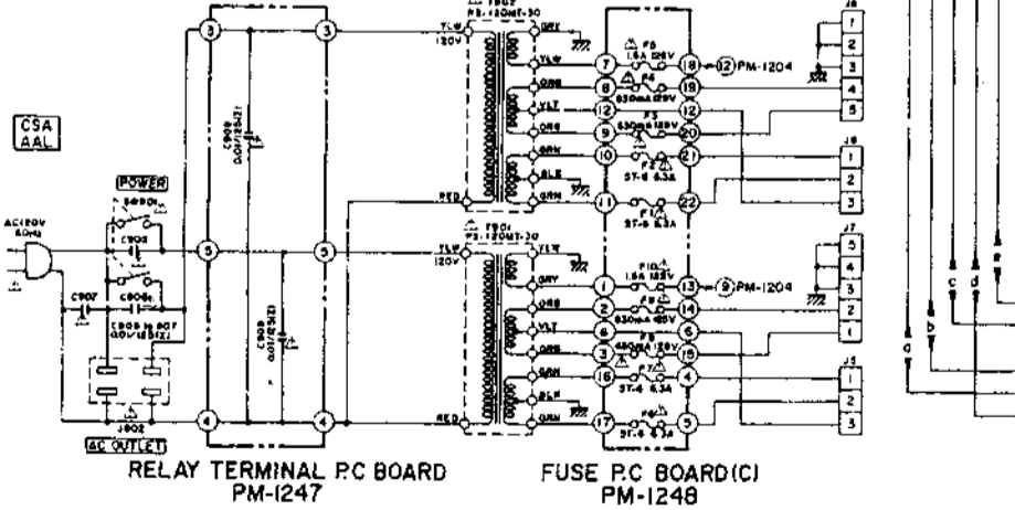
RELAY TERMINAL P.C. BOARD PM-1247
