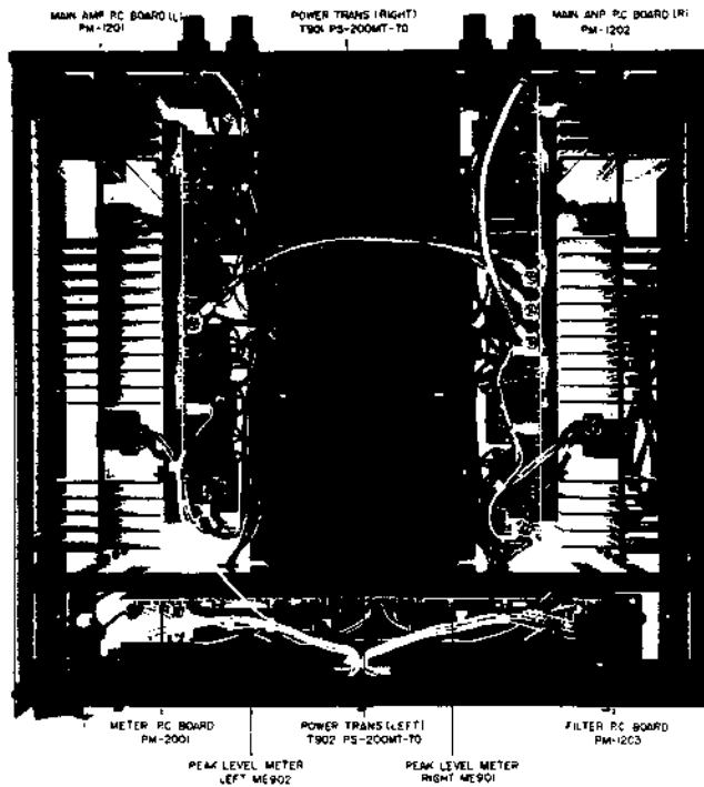
Fig. 7 Top View
