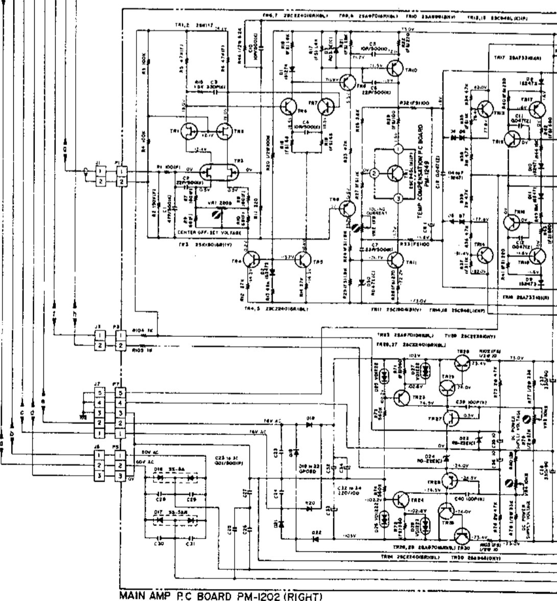
MAIN AMP P.C. BOARD PM-1202 (RIGHT)
