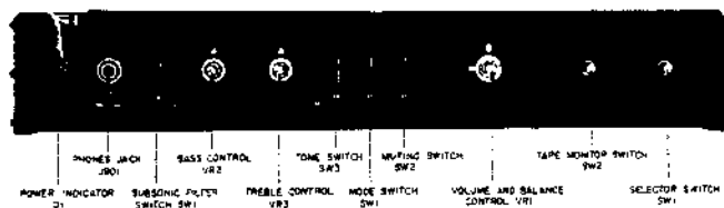
Fig. 4 Front View
