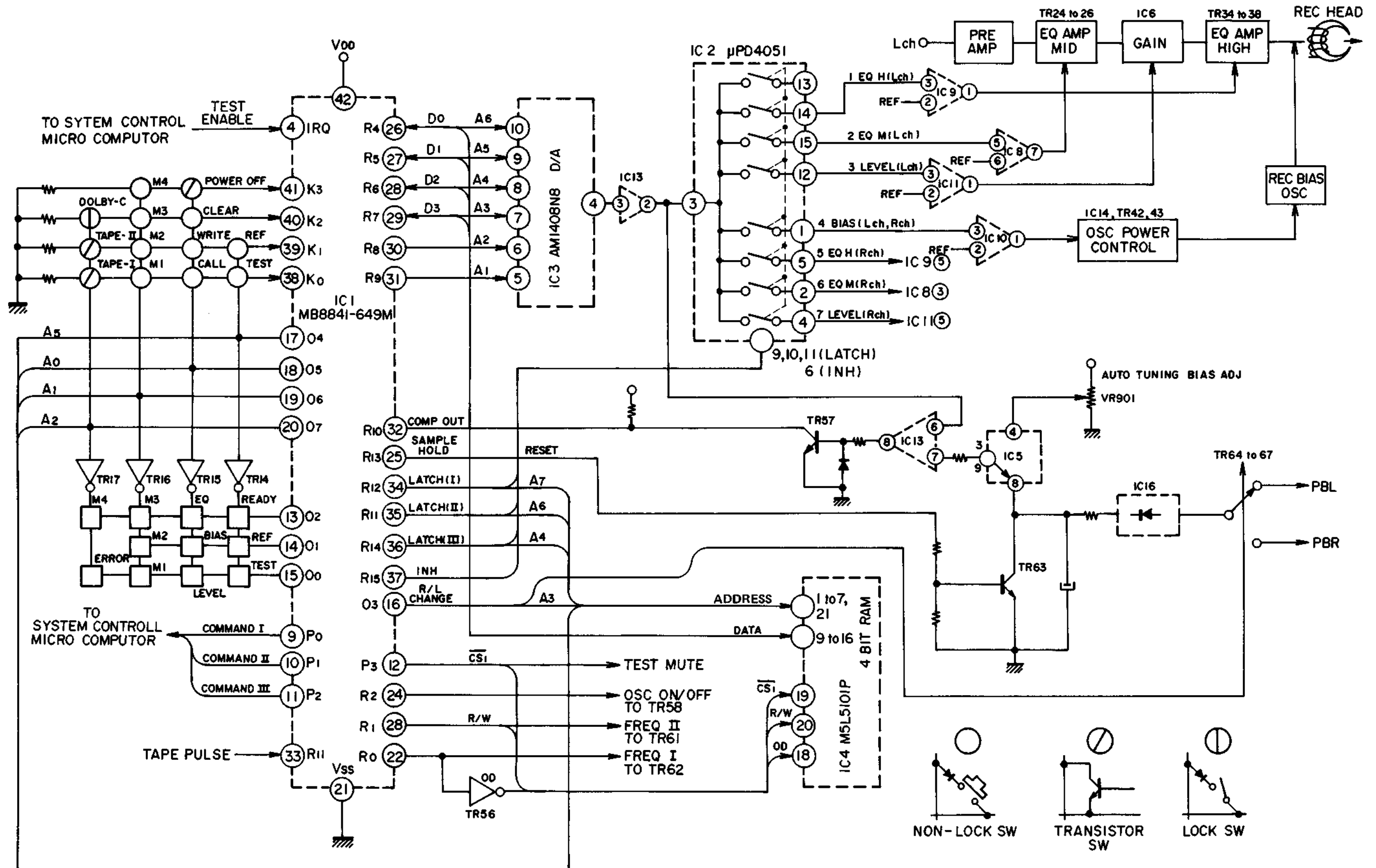
Fig. 1-3 Auto Tuning Block Diagram
