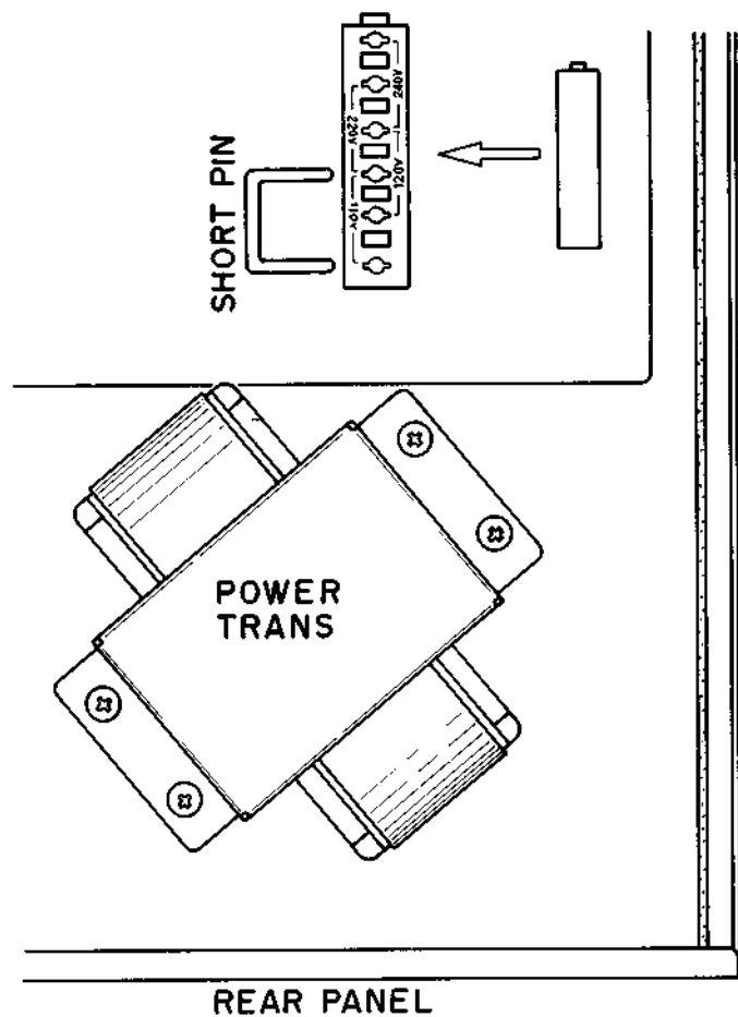
Fig. 2-8 Voltage Conversion (U Model)
