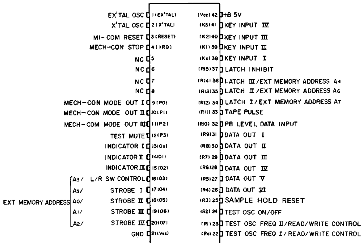
Fig. 1-4 IC1 MB8841-649M
