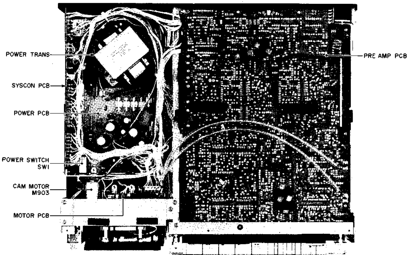
Fig. 2-6 Top View
