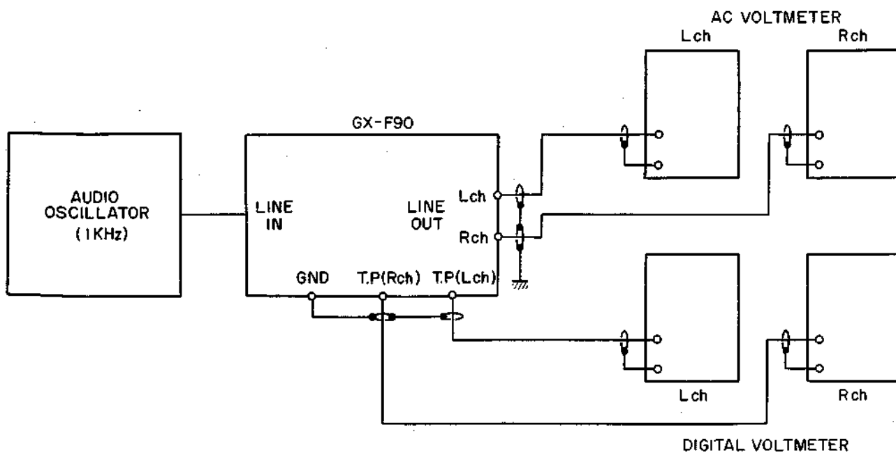
Fig. 28 Instrument Connection
