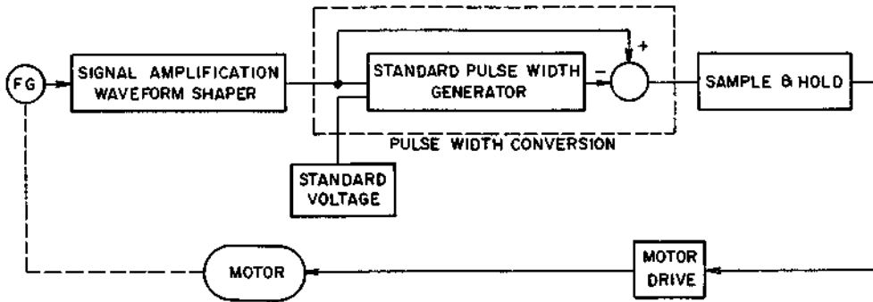
Fig. 14 Servo Circuit Block Diagram
