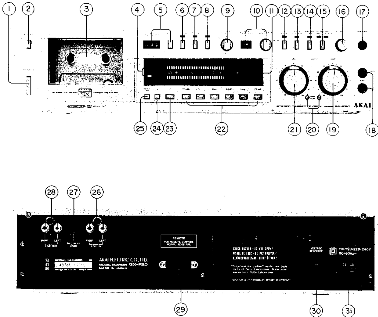
Fig. 1 Controls
