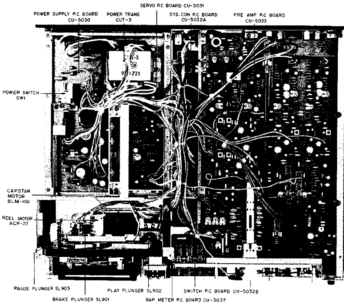
Fig. 3 Top View
