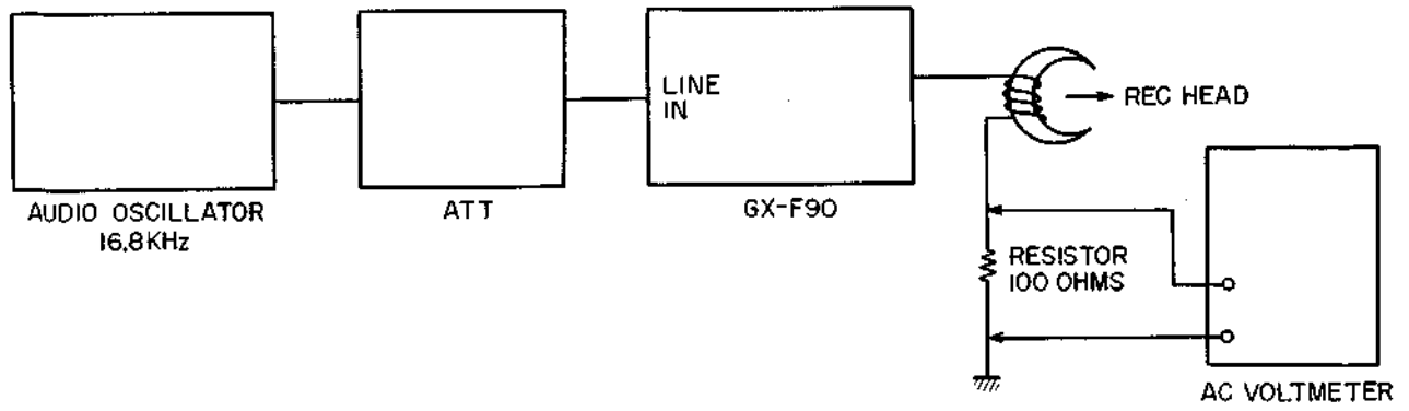
Fig. 25 Instruments Connection
