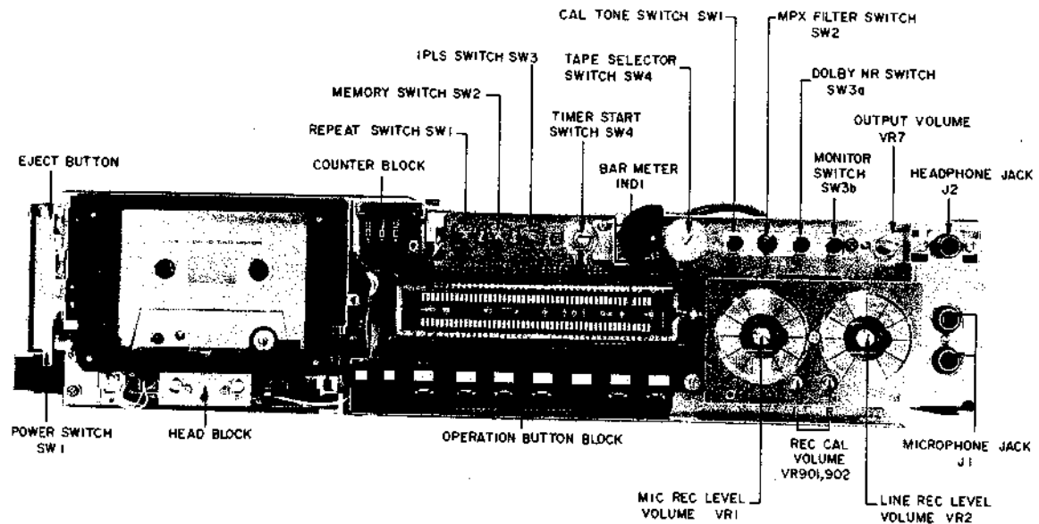
Fig. 2 Front View
