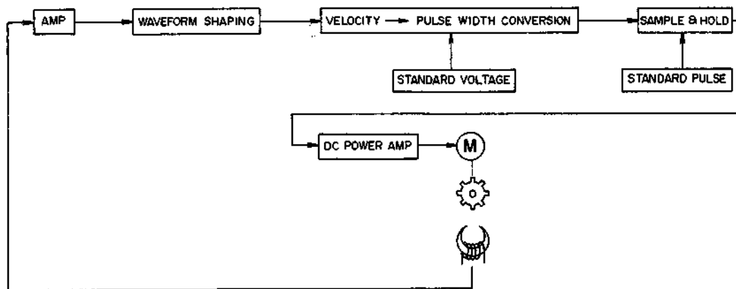
Fig. 5 Block Diagram
