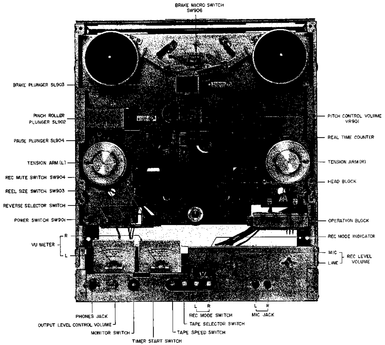
Fig. 2 Front View
