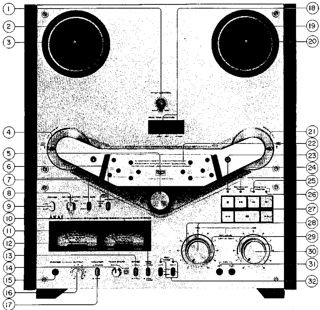
Fig. 1 Controls
