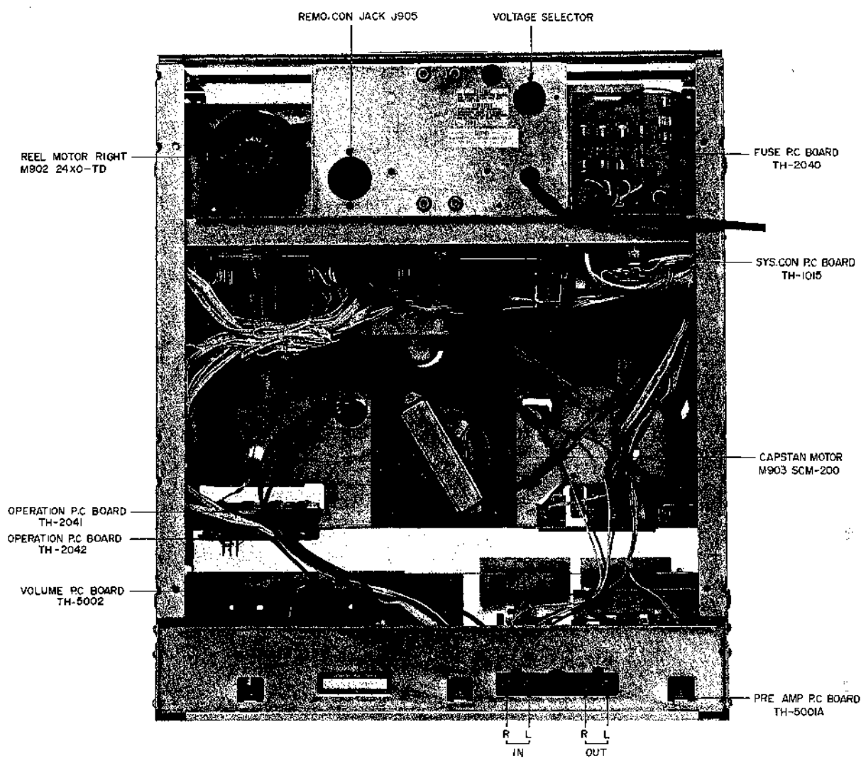
Fig. 3 Rear View
