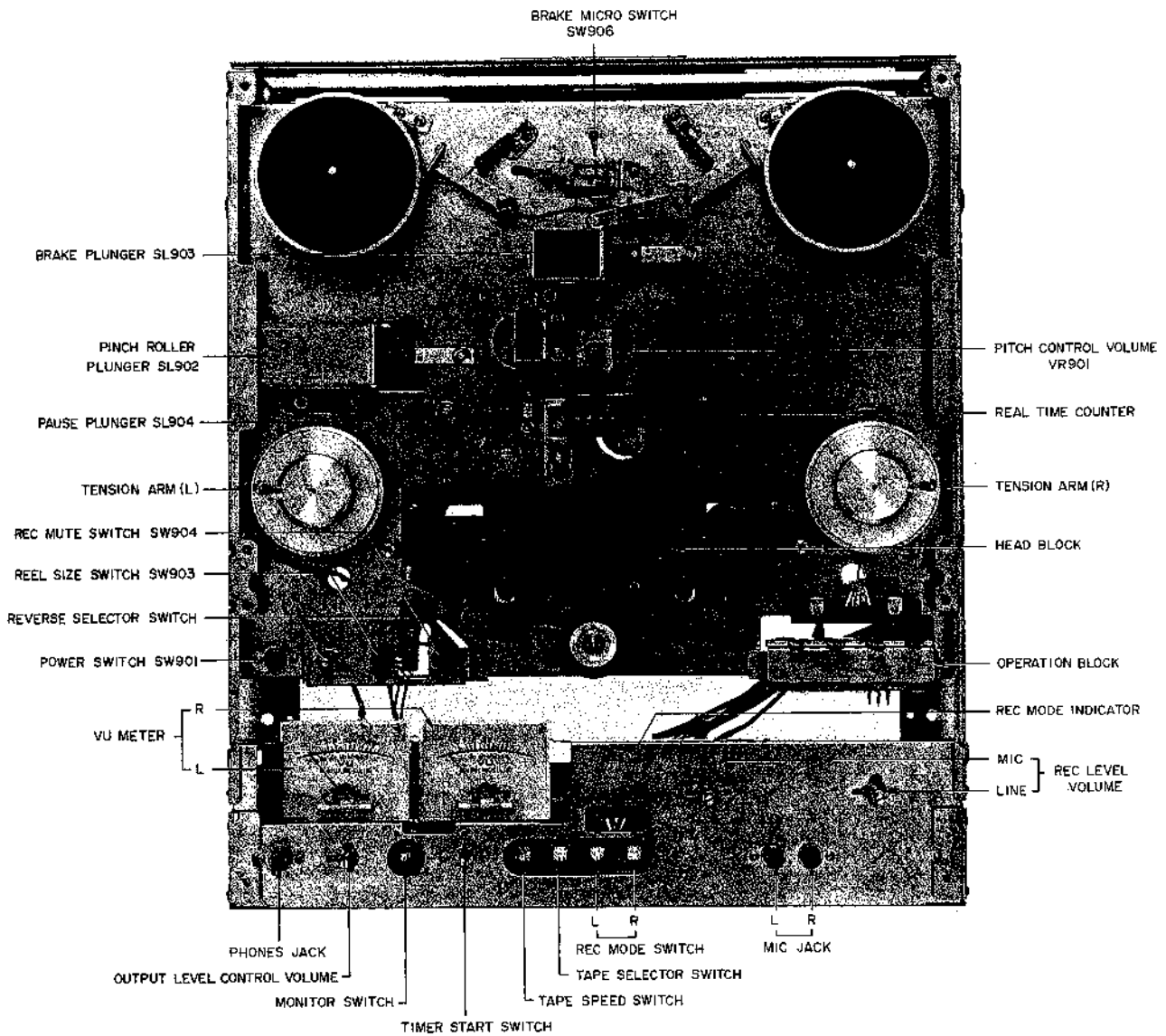
Fig. 2 Front View
