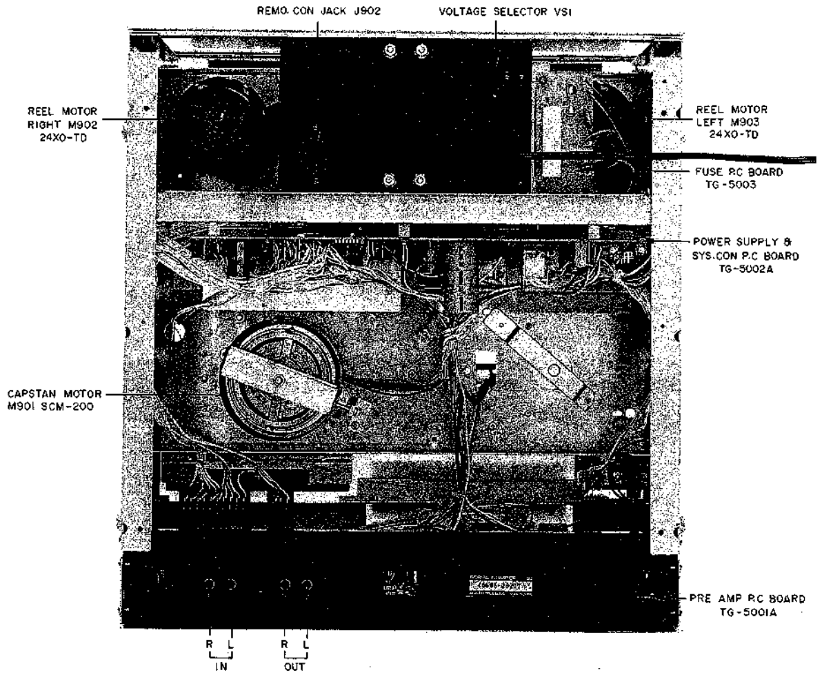
Fig. 3 Rear View
