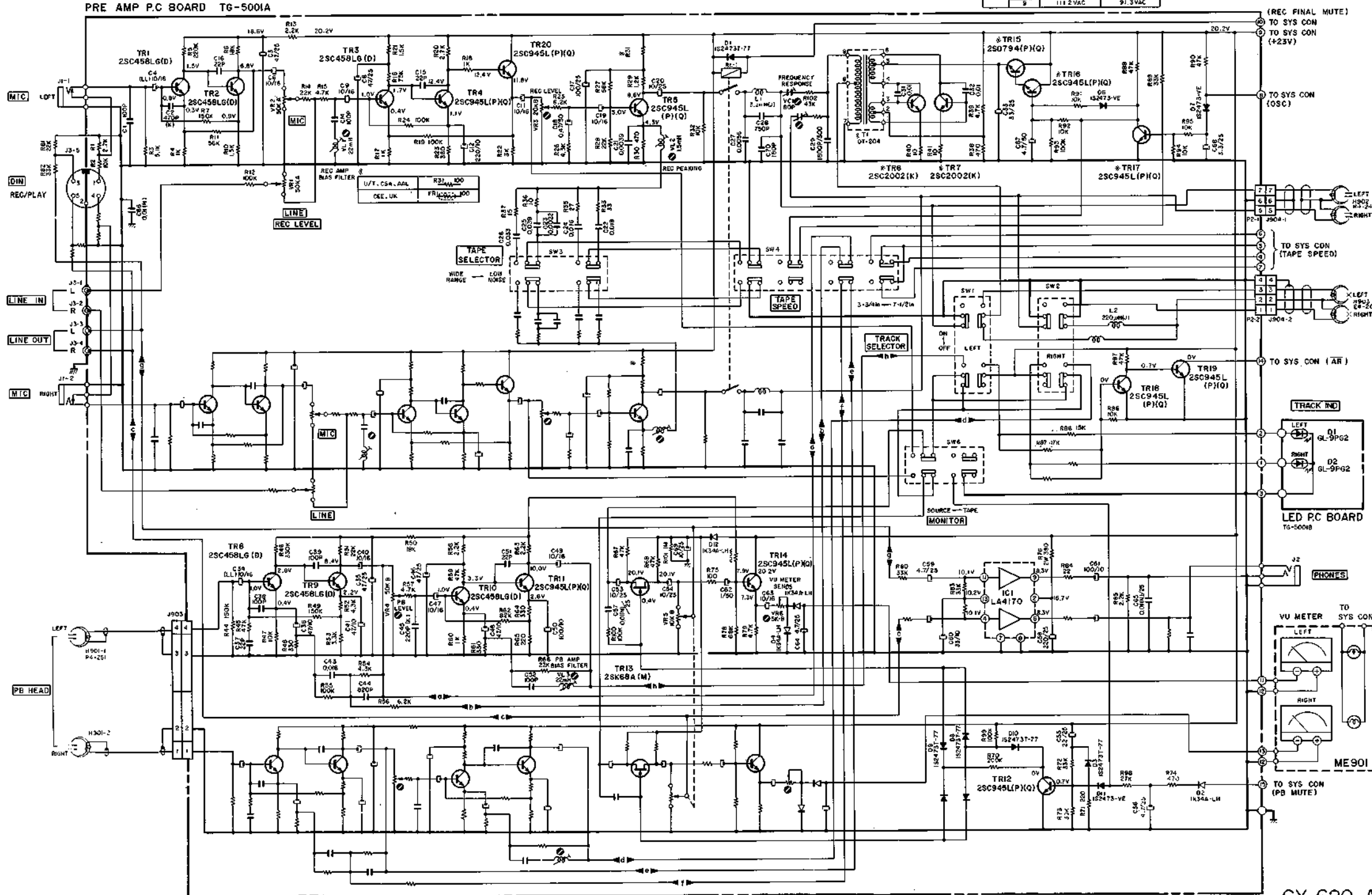
GX-620 AMP SCHEMATIC DIAGRAM NO.2-2 1582039A
