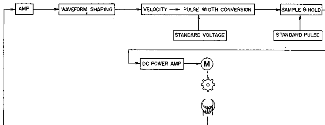
Fig. 7 Block Diagram
