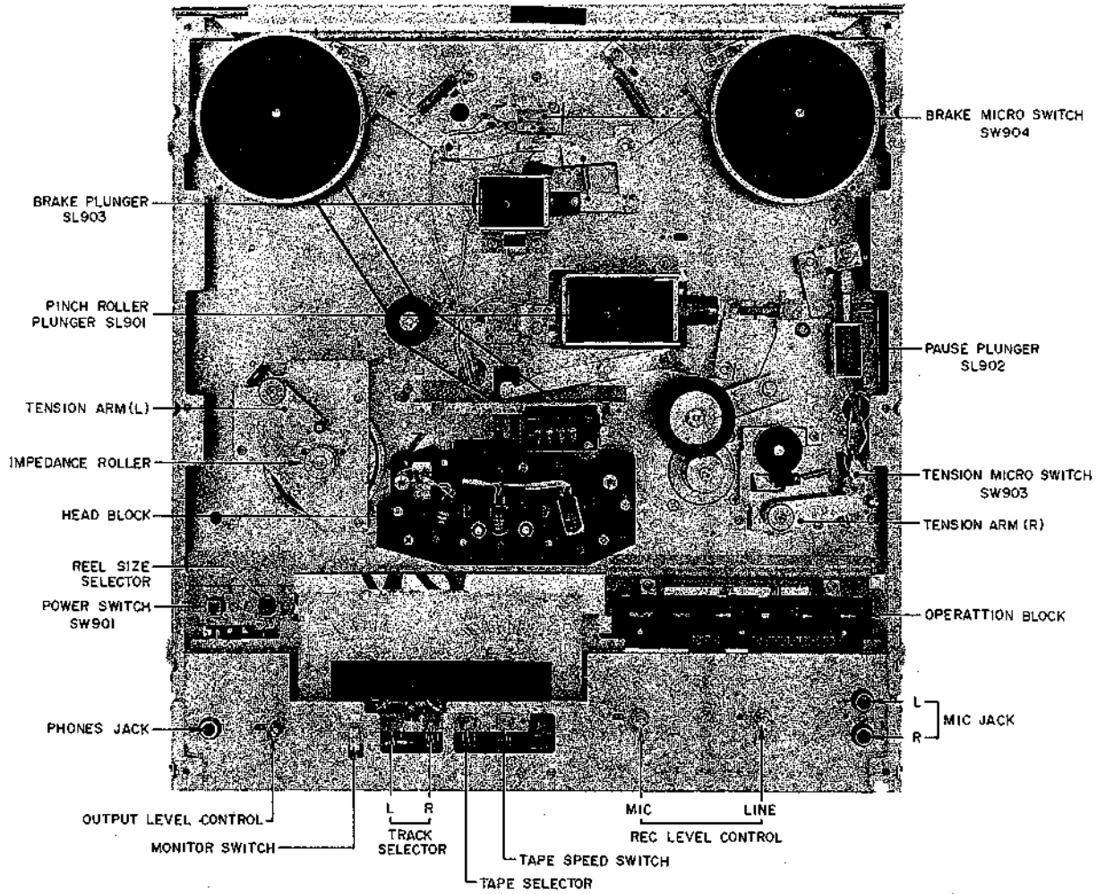
Fig. 2 Front View
