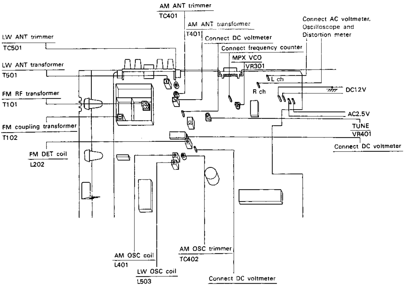
Fig. 12-3 Adjustment positions
