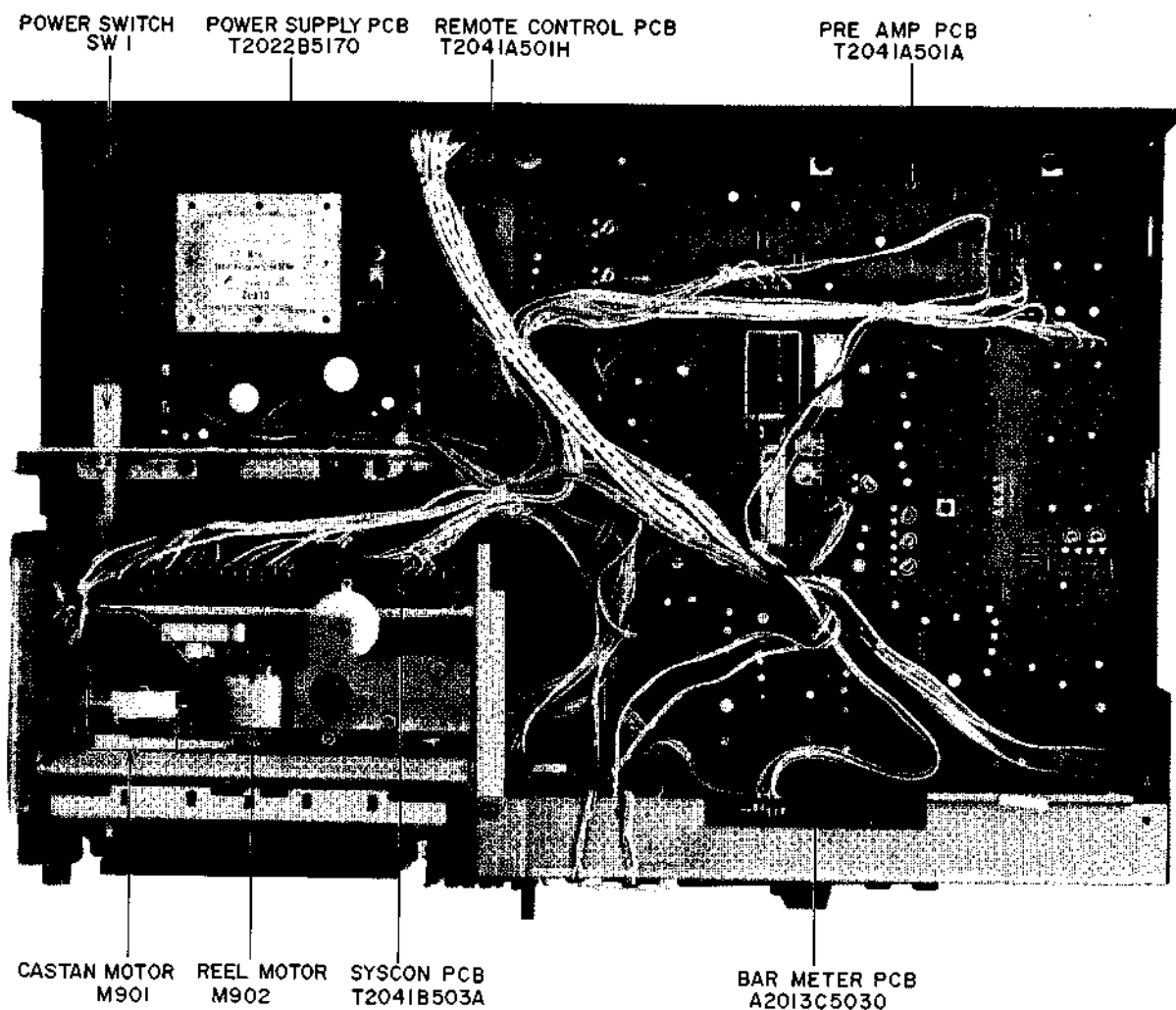
Fig. 6 Top View
