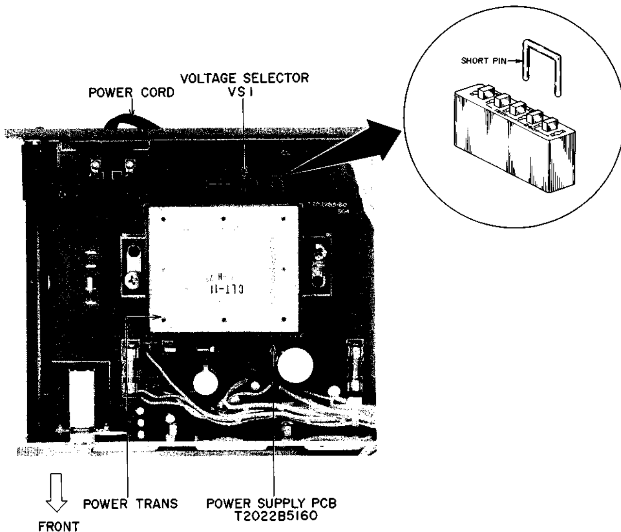
Fig. 7 Voltage Conversion (U/T Model only)
