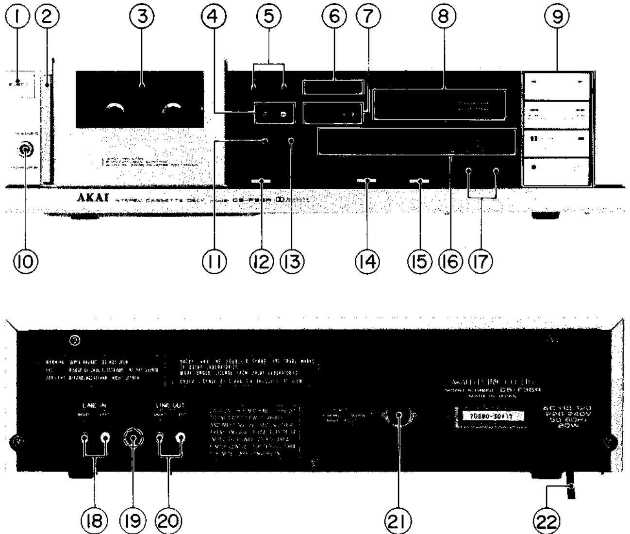
Fig. 1 Controls
