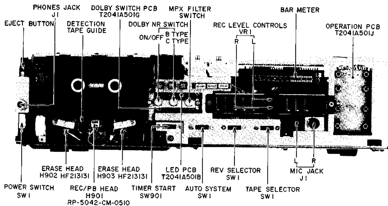
Fig. 5 Front View
