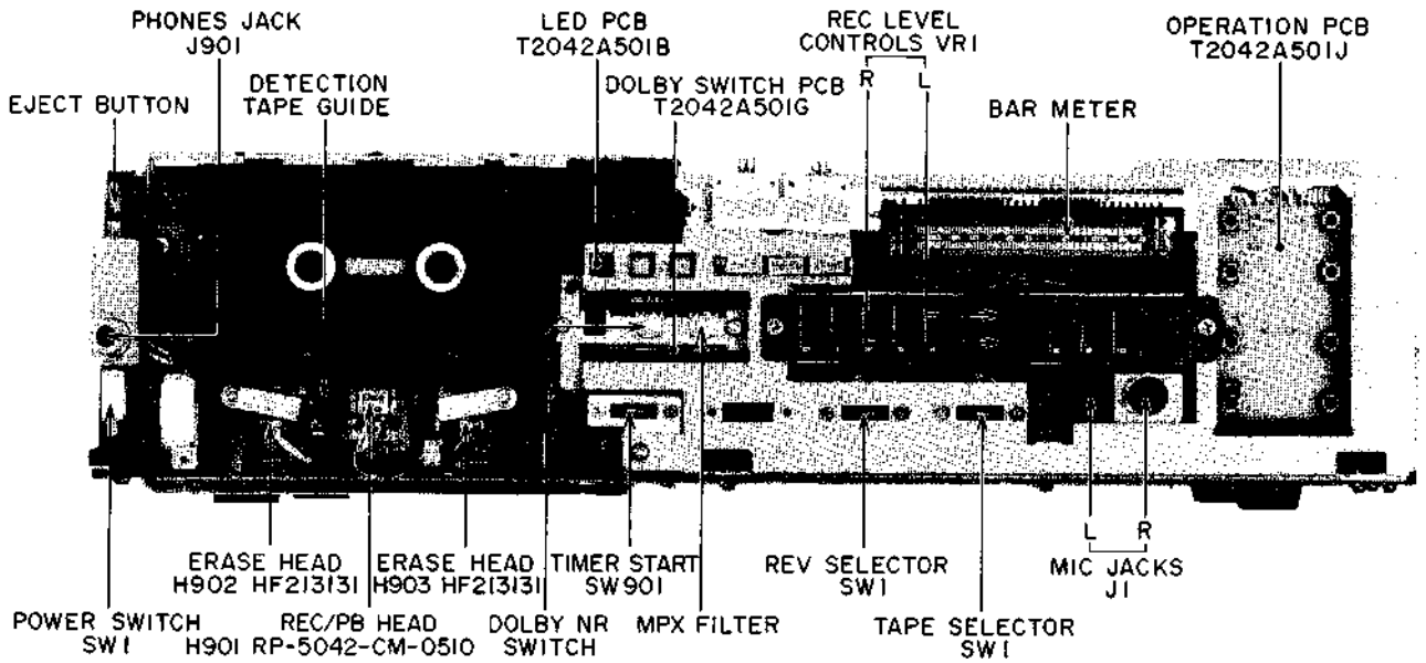
Fig. 3 Front View
