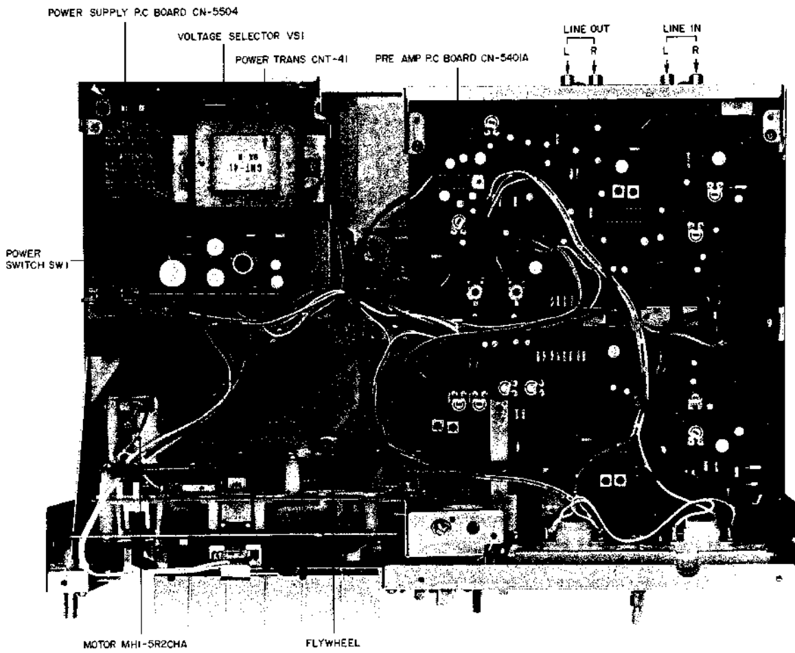
Fig. 5 Top View
