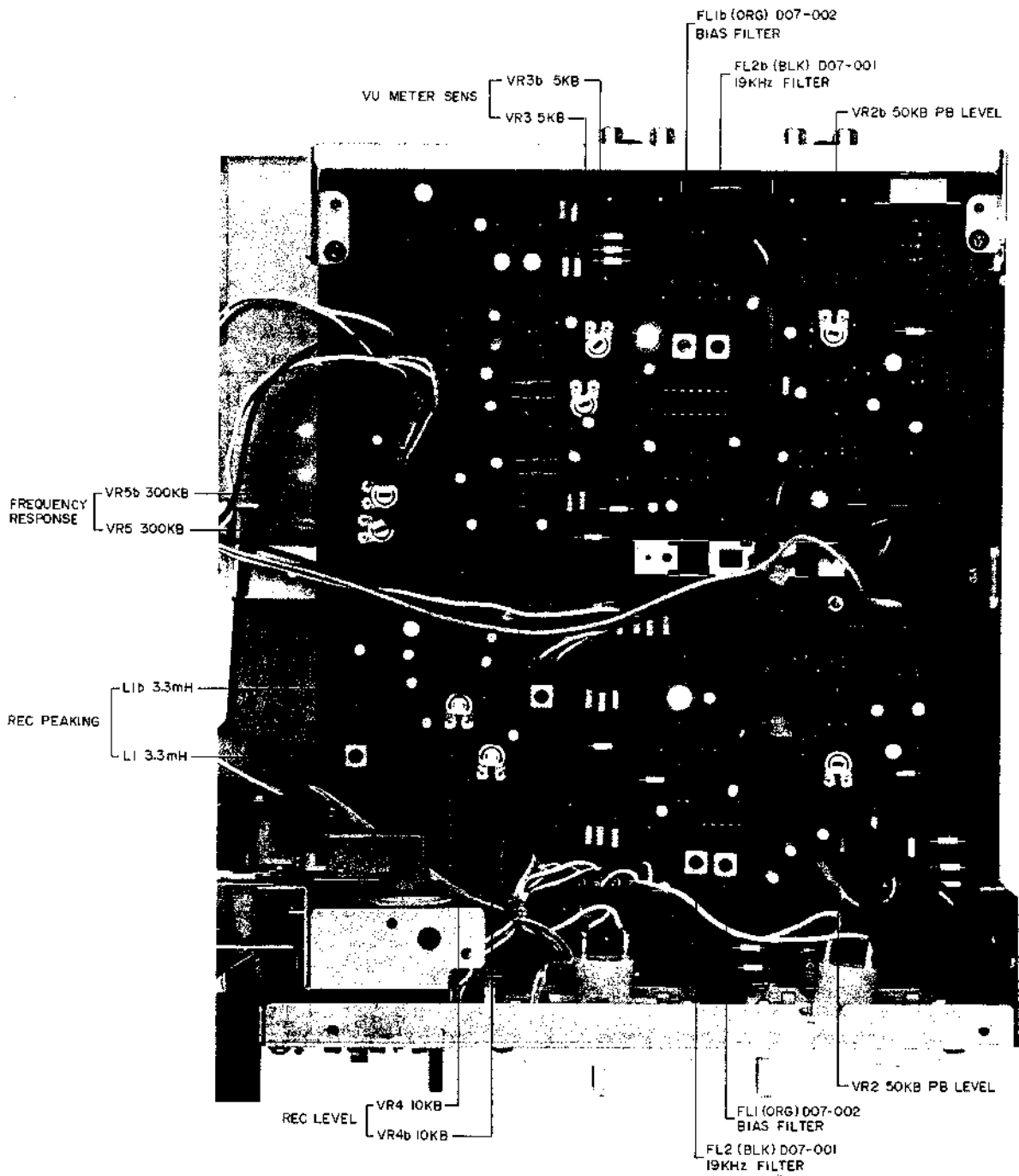
Fig. 17 Pre Amp P.C Board CN-5501A
