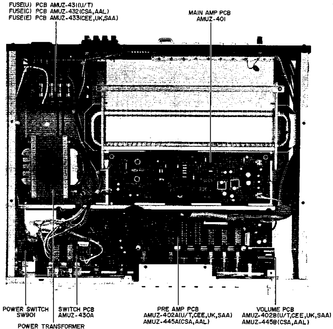
Fig. 4 Top View
