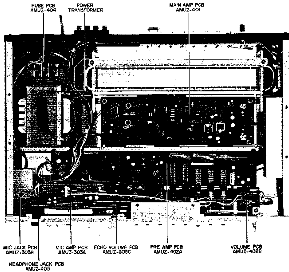
Fig. 6 Top View
