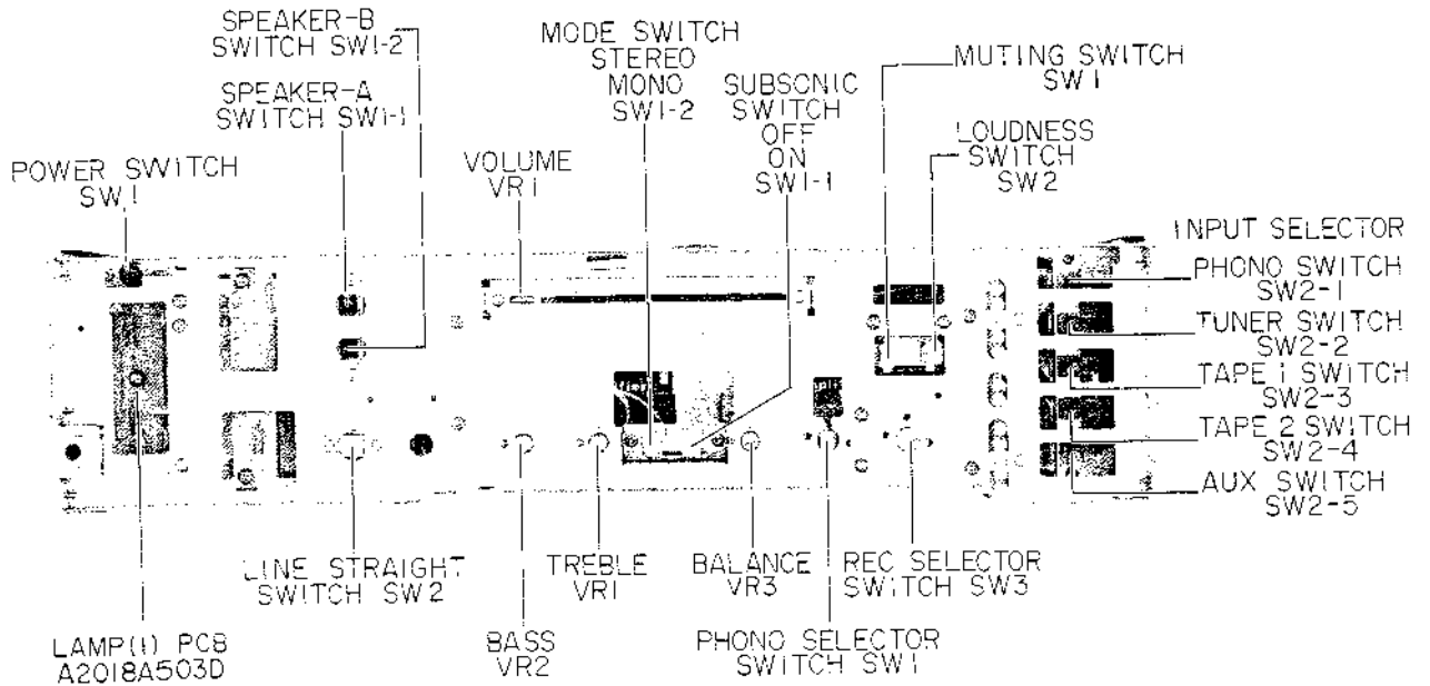
Fig. 3 Front View
