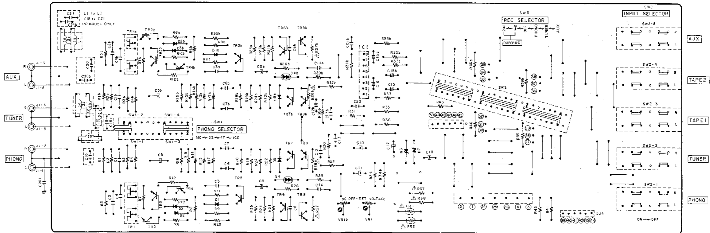
EQUALIZER PCB A2018A501A
