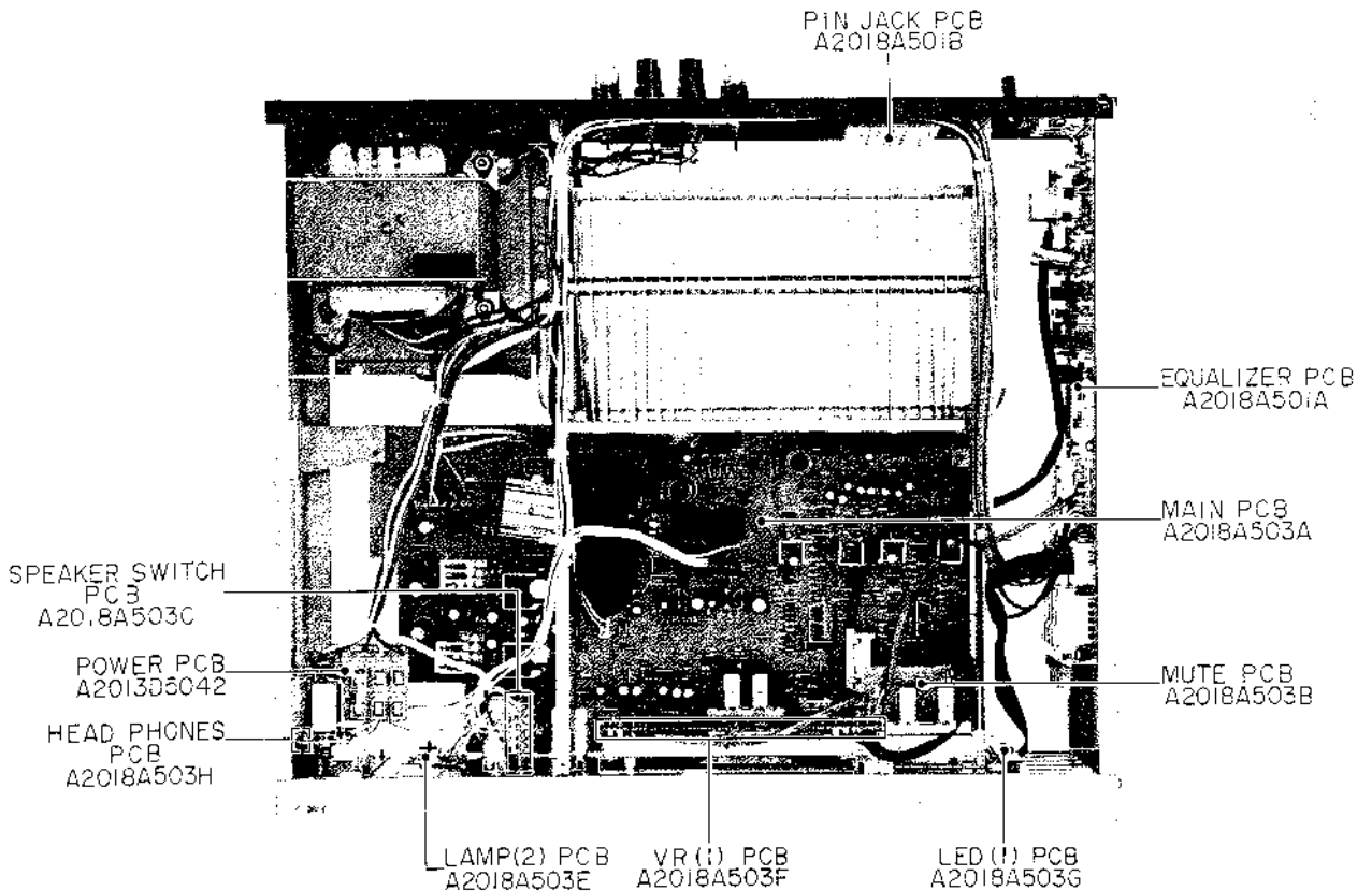
Fig. 4 Top View
