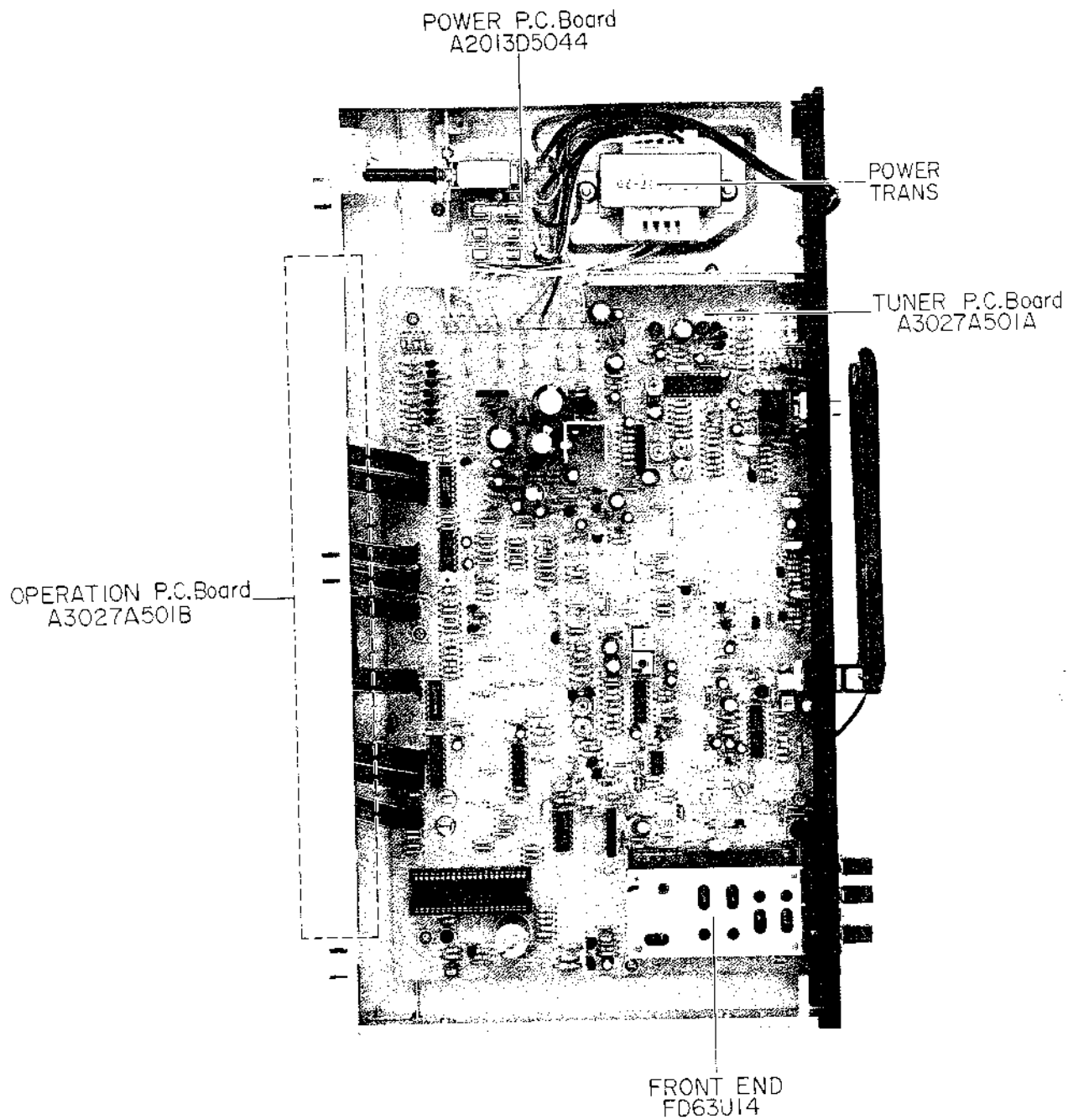
Fig. 2 Top View
