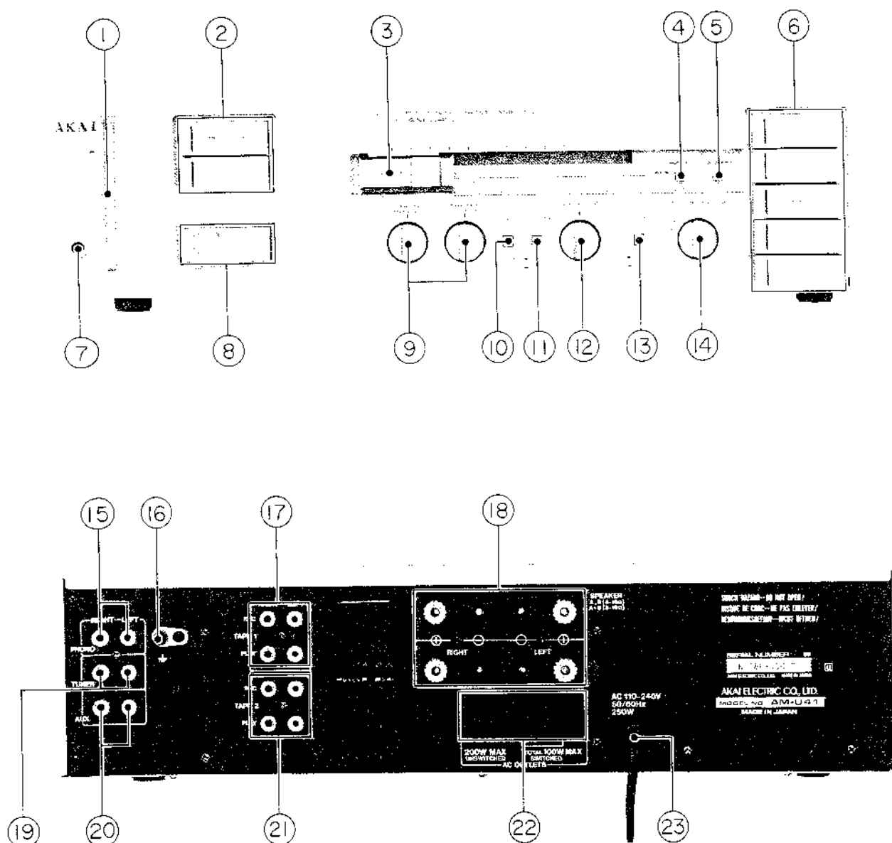
Fig. 1 Controls
