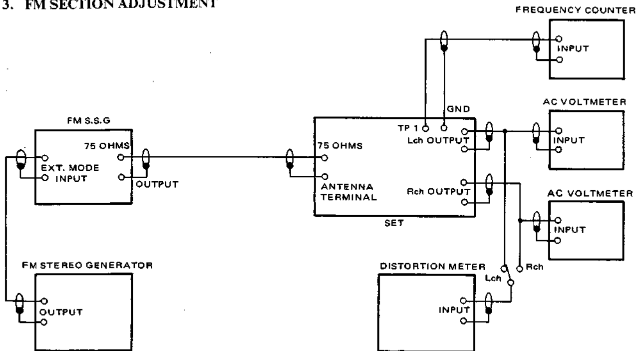
Fig. 13 Instruments Connection for FM Section Adjustment
