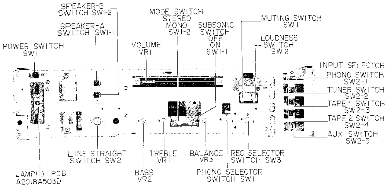
Fig. 5 Front View
