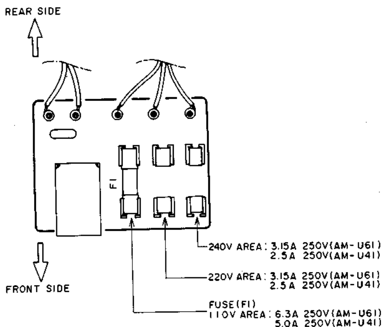
Fig. 7 Voltage Conversion (U Model only)
