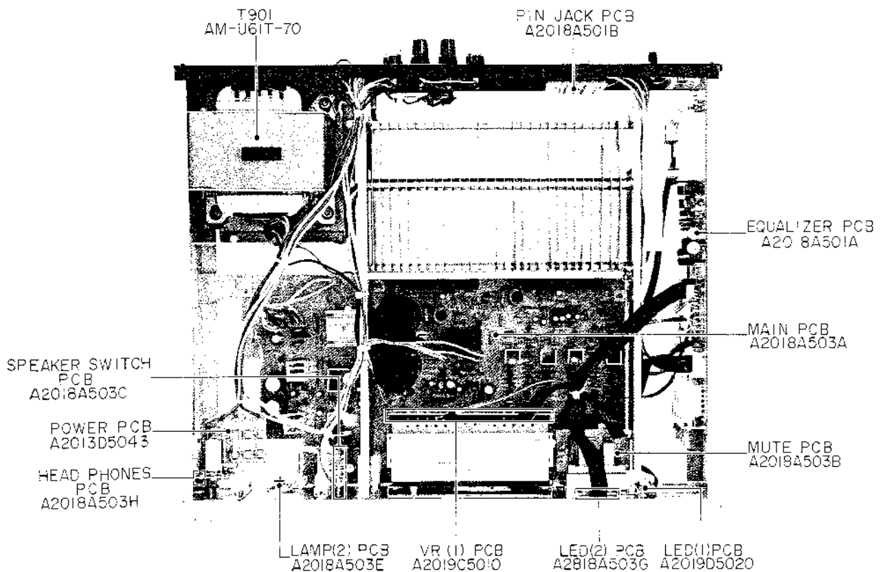
Fig. 6 Top View
