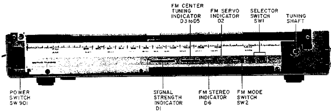
Fig. 2 Front View
