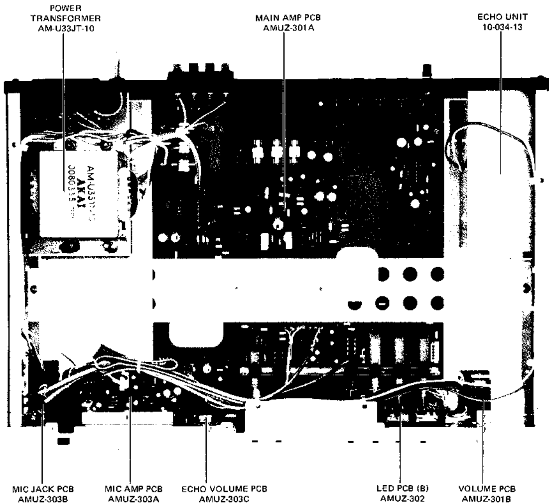
Fig. 3 Top View
