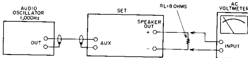
Fig. 5 Instrument Connections
