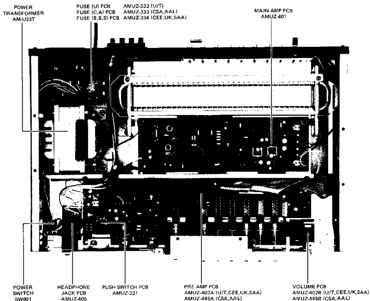
Fig. 3 Top View
