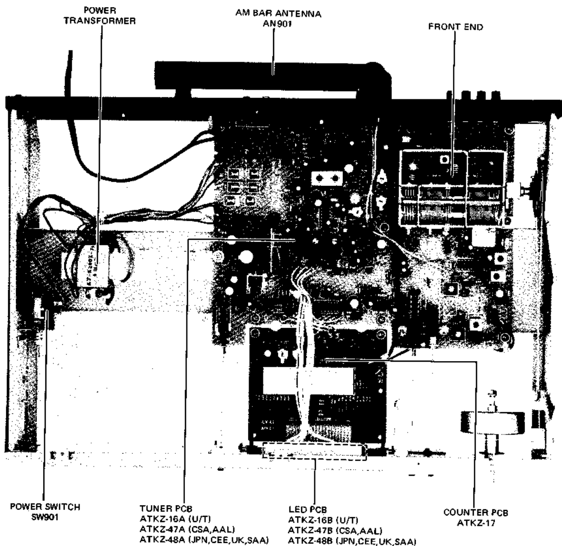
Fig. 3 Top View
