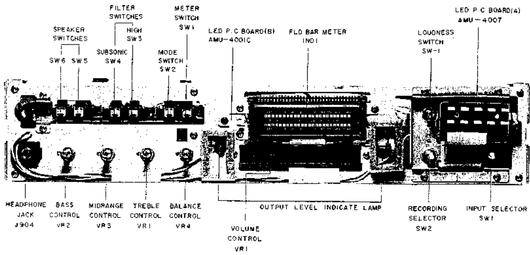
Fig. 2 Front View
