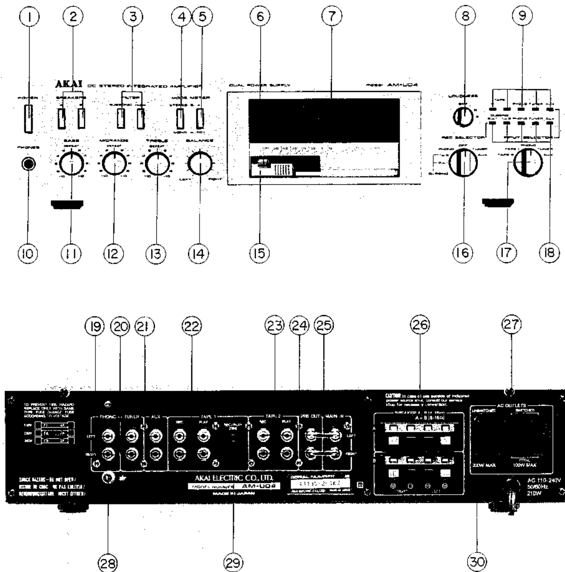
Fig. 1 Controls
