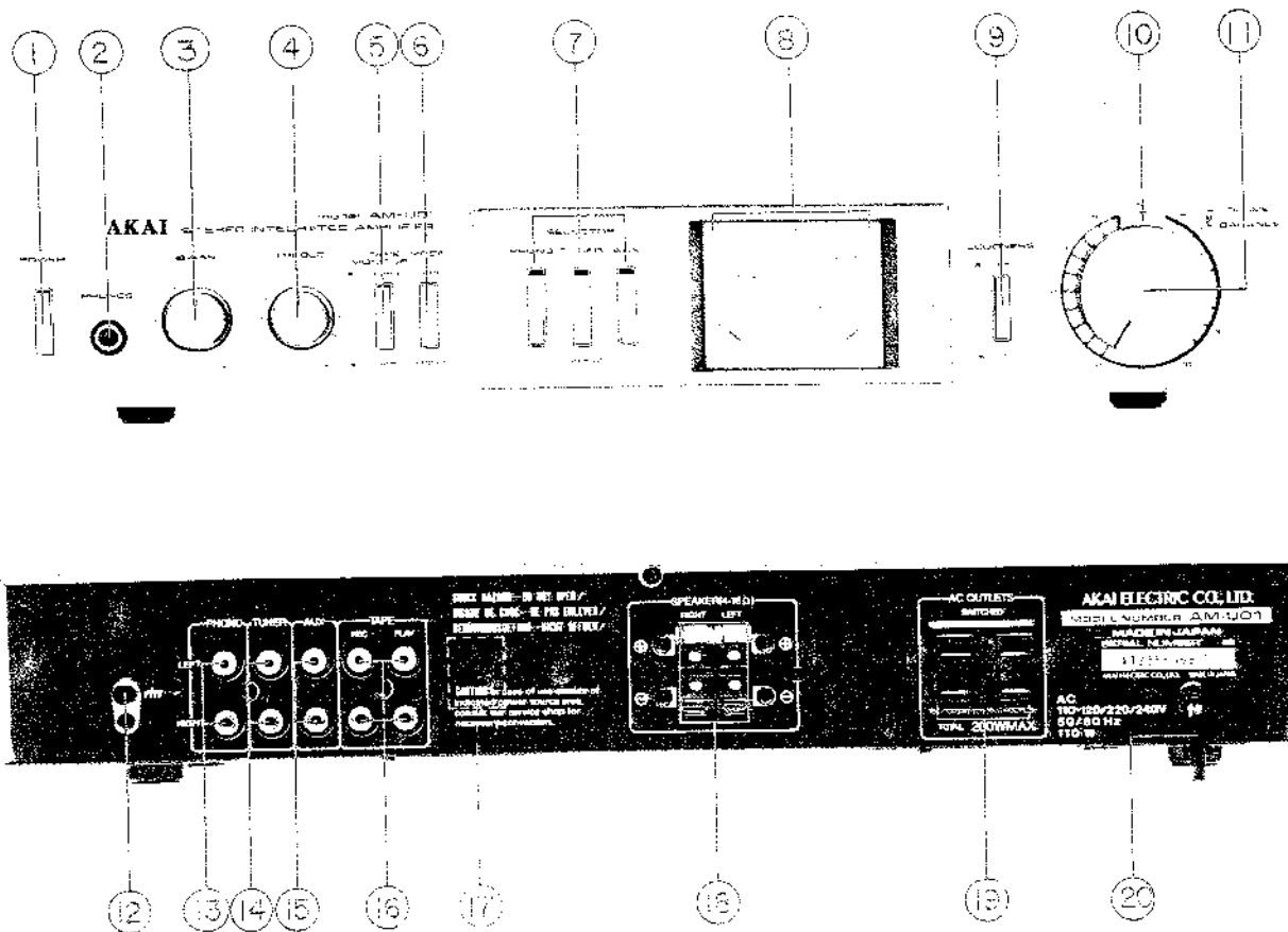
Fig. 1 Controls
