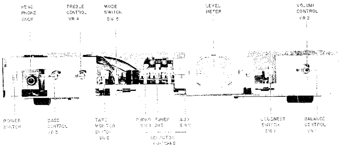
Fig. 2 Front View
