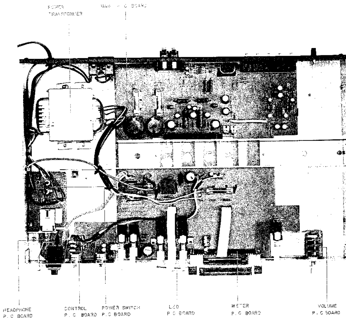
Fig. 3 Top view
