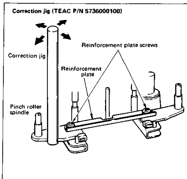
Fig. 2-19 Pinch roller/capstan alignment
