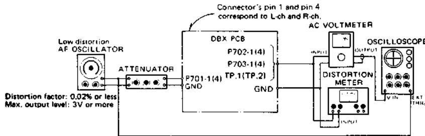
Fig. 3-13 Decoder adjustment setup
