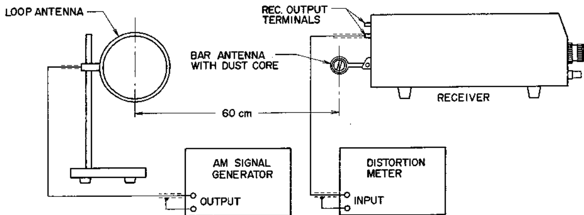
Fig. 16 INSTRUMENT CONNECTIONS
