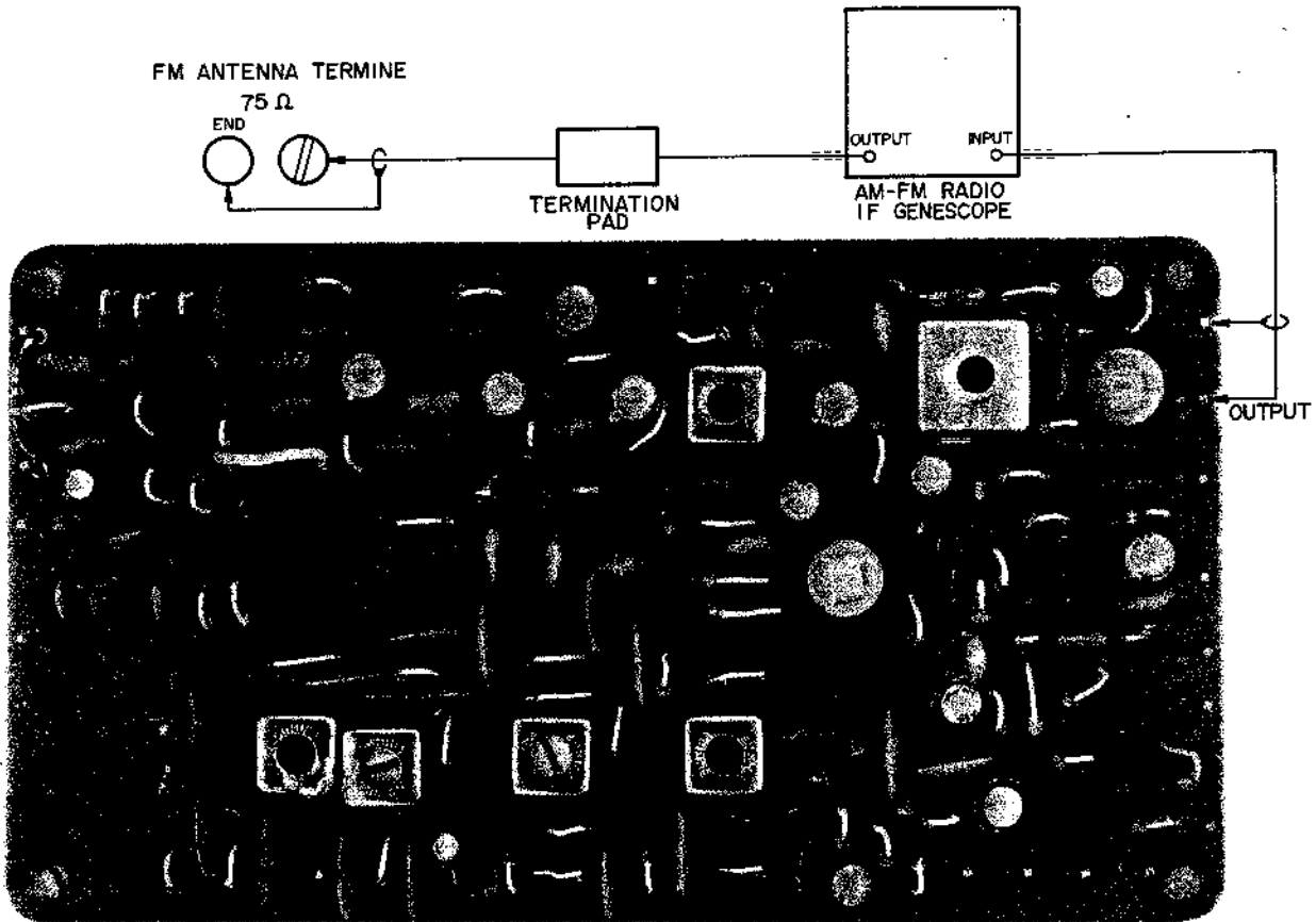
Fig. 7 INSTRUMENT CONNECTIONS
