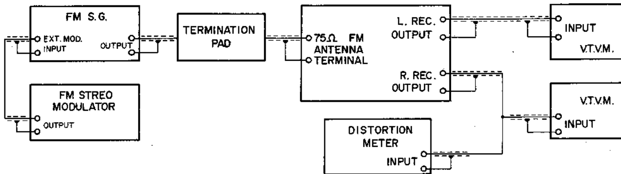
Fig. 11 INSTRUMENT CONNECTIONS
