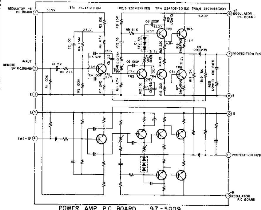
POWER AMP. P.C. BOARD 97-5009
