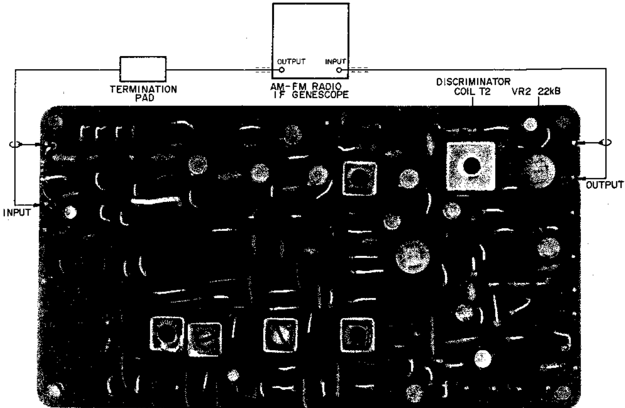
Fig. 3 INSTRUMENT CONNECTIONS
