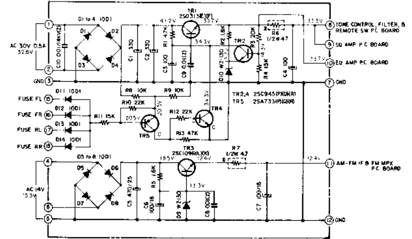
REGULATION P.C. BOARD 98-5084
