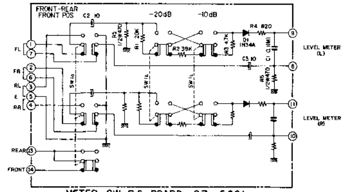
METER SW P.C. BOARD 97-5001
