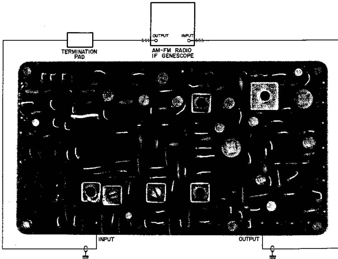
Fig. 14 INSTRUMENT CONNECTIONS
