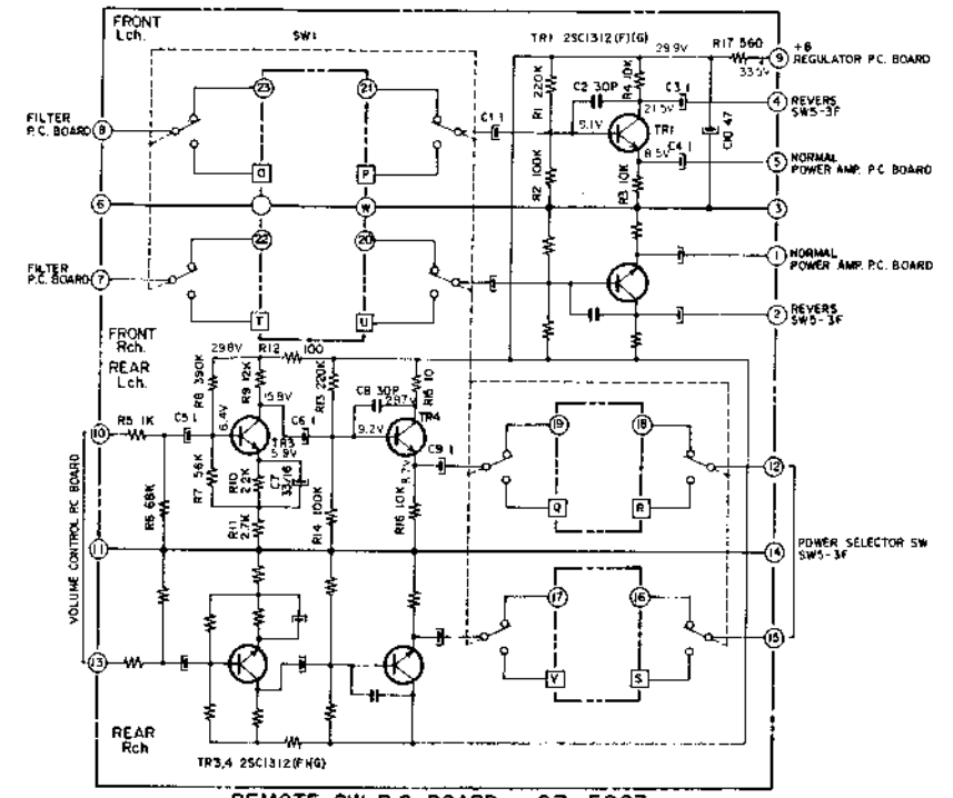
REMOTE SW P.C. BOARD 97-5003
