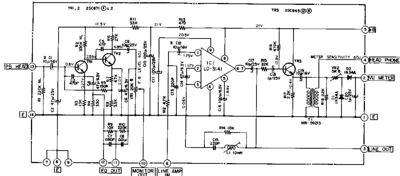
P. B. AMP P. C. BOARD KH-5014
