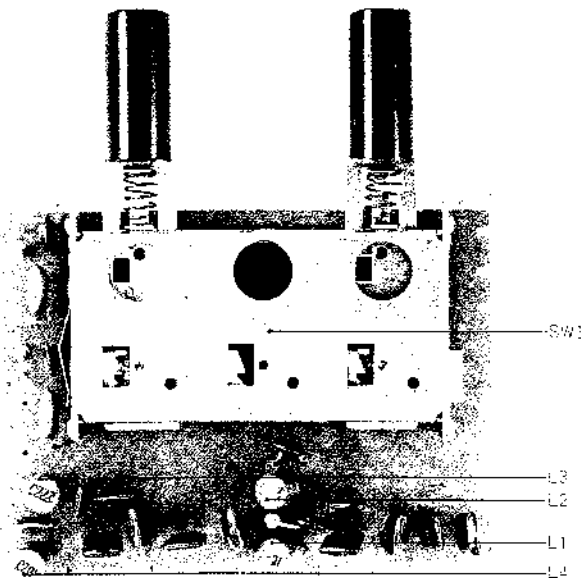
FIG. 9 PHOTO OF TAPE SPEED SWITCH P.C. BOARD (KH-2011)
