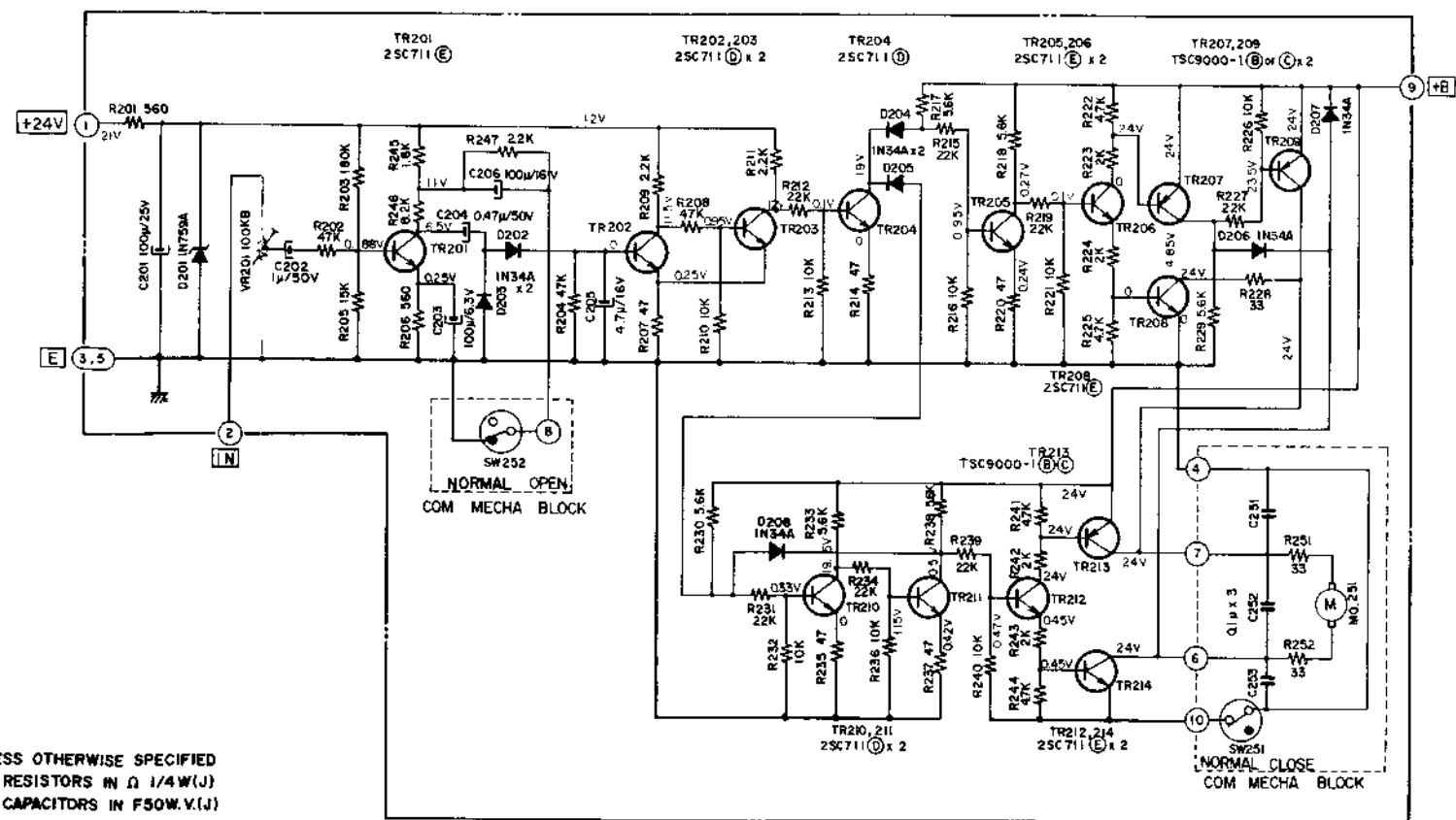
COM DET P. C. BOARD RD-A514
