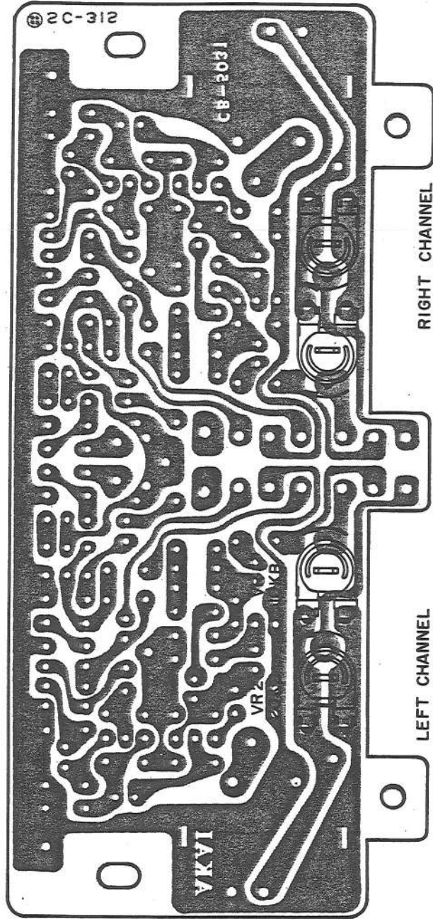
Fig-15 PEAK METER PC BOARD CB-5013
