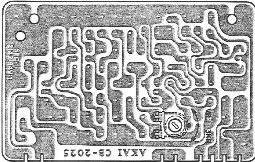
Fig - 10 SERVO P.C BOARD CB-2025
