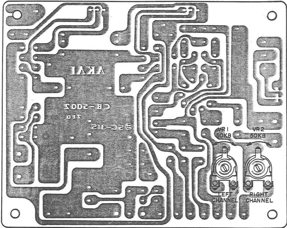
Fig-14 POWER SUPPLY & OSC P.C BOARD CB-5002
