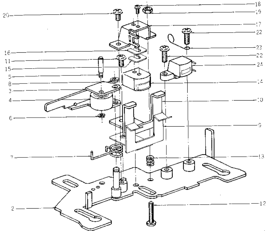
FIG. 1 ILLUSTRATION OF HEAD BASE BLOCK
