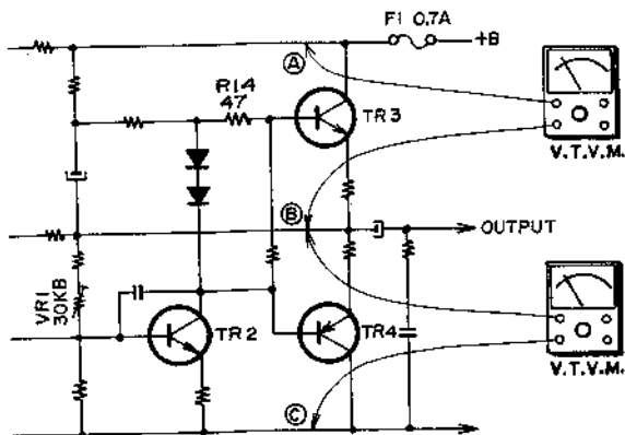
POWER AMP CIRCUIT
