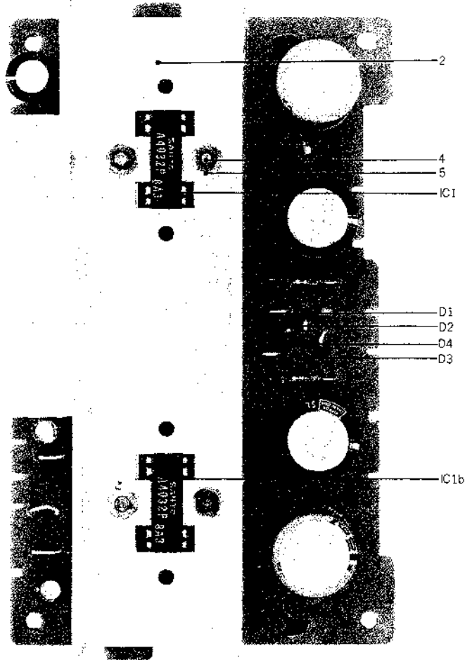
FIG. 10 PHOTO OF MAIN AMP. P.C. BOARD (CG-5403) (GXC-38 UL, J)
