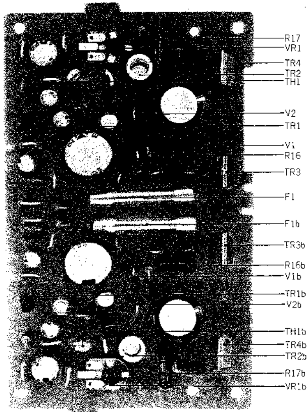
FIG. 9 PHOTO OF MAIN AMP. P.C. BOARD (CG-5009)
