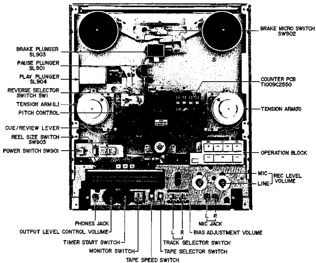
Fig. 2 Front View
