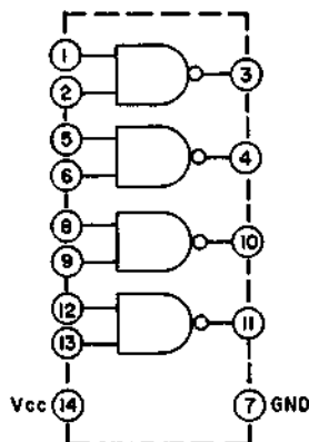
MC14011BCP
