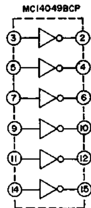
MC14049BCP
