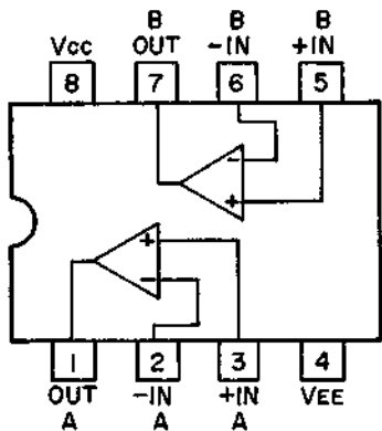
NJM4558D
