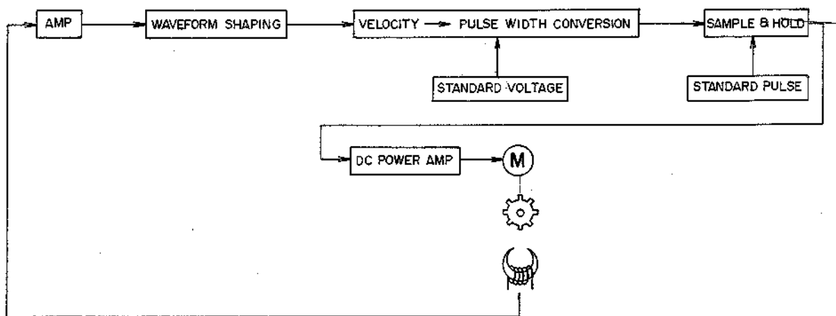
Fig. 19 Block Diagram
