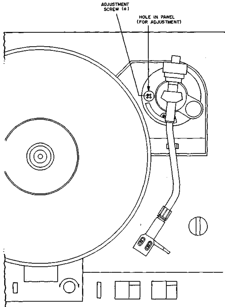
Fig. 21 Lead-in Adjustment
