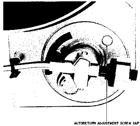
Fig. 8 Auto-Return Adjustment
