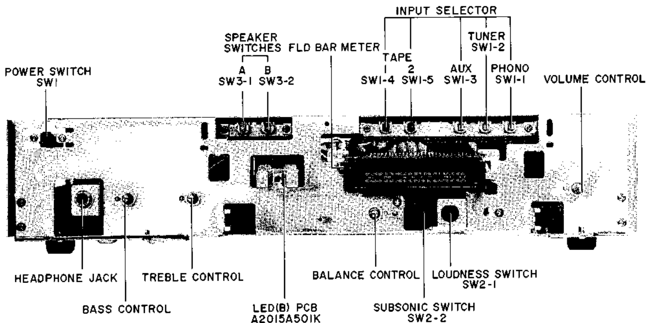
Fig. 2 Front View
