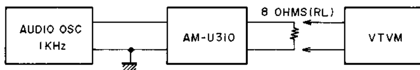
Fig. 6 Instrument Connection for Power Meter Sensitivity
