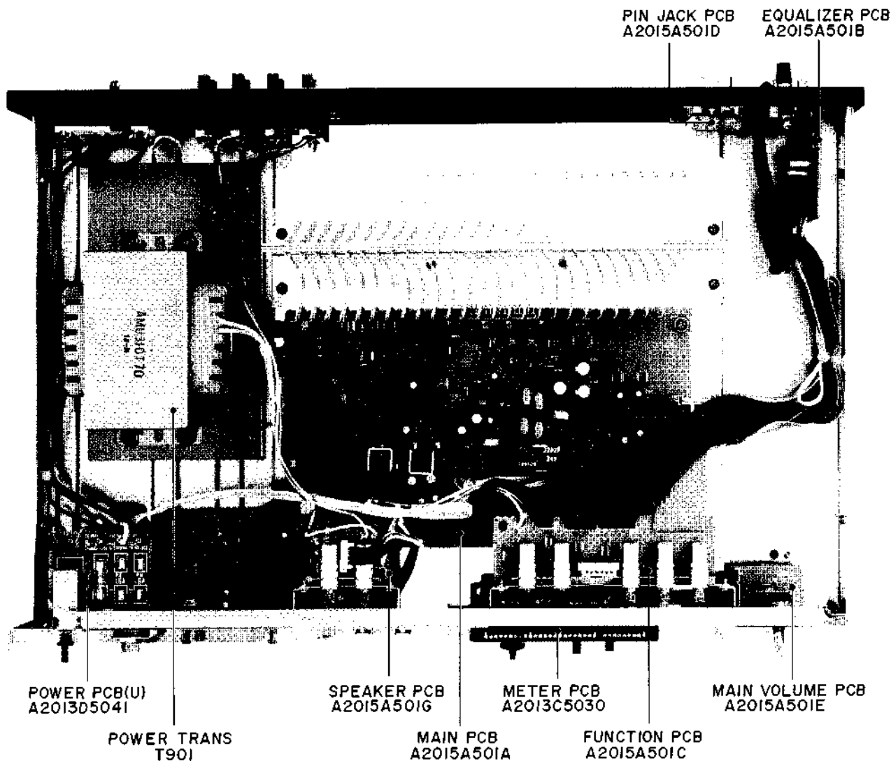
Fig. 3 Top View
